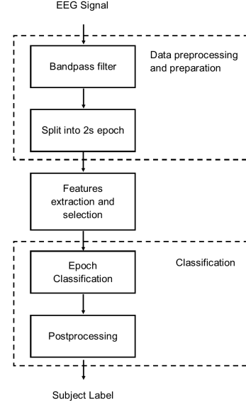
Fig. 1. A high-level overview of the proposed algorithm.
