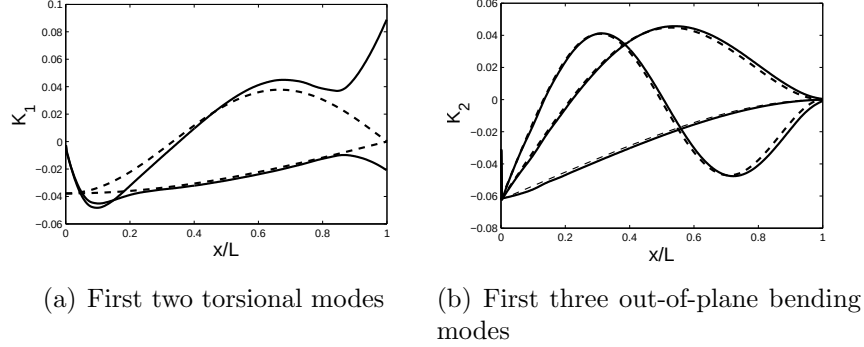
Figure 5: Curvature of the mode shapes, \mathbf{C}\Phi_{2j} , as obtained from 3-D FEM (continuous lines) and the constant-section beam model (dashed).
