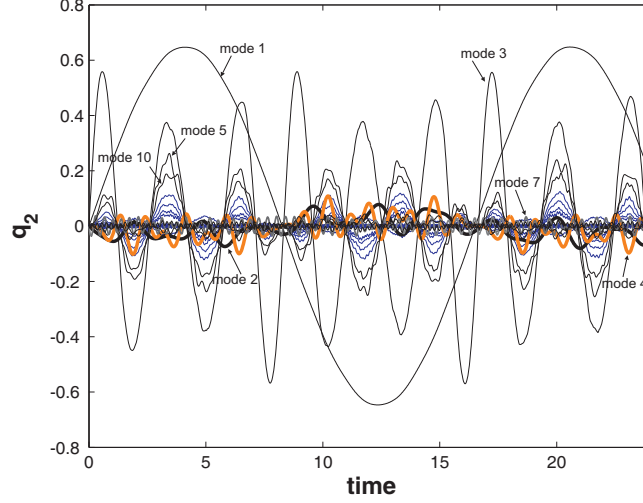
Figure 8: First 20 modal amplitudes of the force component q_2 for \mathbf{x}_{10} = (0; 2; 2; 0; 0; 0) . Modes 11-20 are shown in blue and all visible modes from Table 1 have been identified.
