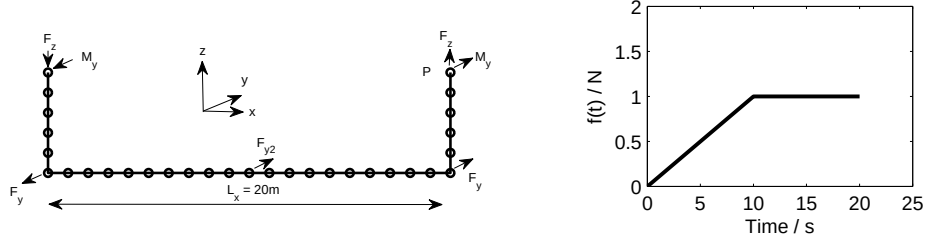
(a) Initial configuration of the structure shown with 31 nodes. Applied forces and moments are also indicated.
