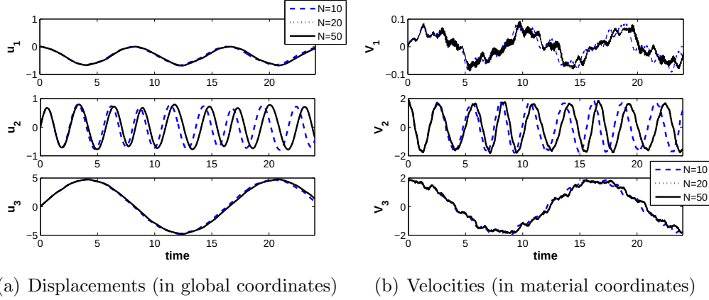
Figure 7: Displacements and velocities at x = L for large initial velocities, \mathbf{x}_{10} = (0; 2; 2; 0; 0; 0) , and increasing number of LNMs in the nonlinear intrinsic model.
