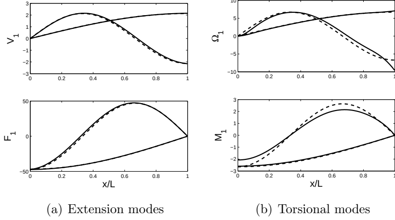
Figure 4: First two axial and torsional modes in intrinsic coordinates from the reduction from 3-D FEM (continuous lines) and the constant-section beam model (dashed)
