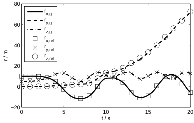
Figure 17: Comparison of the response in Figure 16 for the spatial location of point P in Figure 10(a) for the reduced model from static condensation ( \mathbf{r}_g ) and converged solution from SAMCEF Mecano ( \mathbf{r}_{ref} ).
