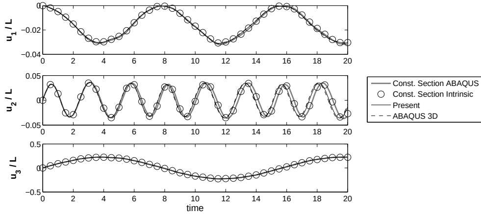
Figure 9: Components of the displacements (in the global frame) at x = L , for \mathbf{x}_{10} = (0; 2; 2; 0; 0; 0) .
