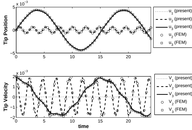
Figure 6: Displacements and velocities at the free end for small initial velocities \mathbf{x}_{10} = (0; 0.002; 0.002; 0; 0; 0) . Results from Nastran (FEM) and the present condensation method.
