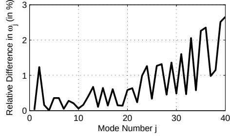
Figure 13: Relative difference in the lowest structural eigenvalues between the condensed system and the beam-element solution for the 31-node model.
