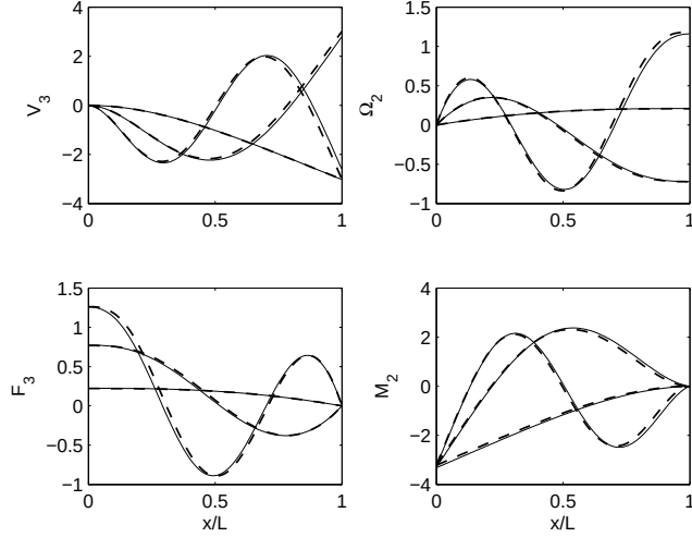
Figure 3: Out-of-plane bending modes in intrinsic coordinates from the reduction from 3-D FEM (continuous lines) and a constant-section beam (dashed).
