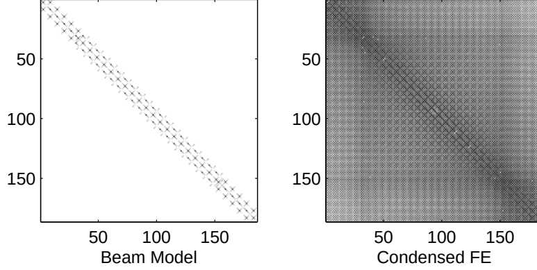
Figure 12: A comparison of sparsity of stiffness matrix \mathbf{K}_a computed from beam elements and a Guyan reduction on 3-D FE model. Both models contain 31 nodes. Dark dots indicate a non-zero entry where shading implies higher magnitude.
