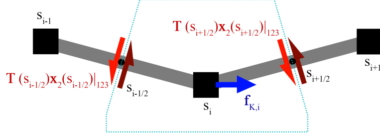
Figure 2: Illustration of the internal forces \mathbf{T}\mathbf{x}_2 (red) and the equivalent nodal applied force \mathbf{f}_{K,i} (blue) at node i for the region outlined by dotted line. The negative sign in one of the internal force terms is due to the definition of the integration direction (in this case equivalent to increasing i ).
