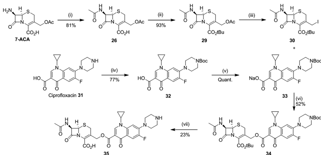
Scheme 1. Synthesis of Prodrug 35 a
