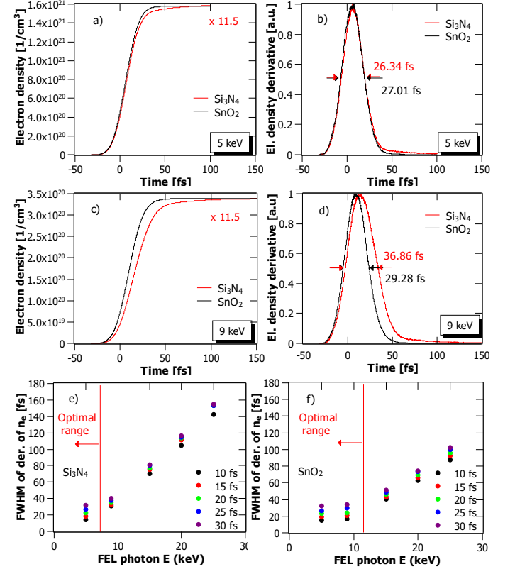
FIG. 1. Calculated evolution of the electron density (a,c), and time derivative of the electron density (b,d) for \text{Si}_3\text{N}_4 and \text{SnO}_2 materials, when irradiated with a 25 fs laser pulse at 5 keV (a,b) and 9 keV (c,d). The electron density function for \text{Si}_3\text{N}_4 was multiplied by 11.5 on both a) and c) for easier comparison. The FWHM of the time derivative of the electron density is plotted to show the optimal range of photon energies where the electron cascading effects happen on a shorter timescale for e) \text{Si}_3\text{N}_4 f) and \text{SnO}_2 , at different photon energies and FEL pulse durations.
