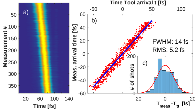
FIG. 3. a) Derivative of the transmission of \text{SnO}_2 at 5 keV. The data has been sorted by the FEL arrival time using our measurement technique: b) Correlation between standard XPP TimeTool diagnostics and our measured arrival time (red measurement points). The blue solid line ( x=y ) is for eye guidance. c) Histogram of the arrival time measurement differences shown for accuracy comparison.
