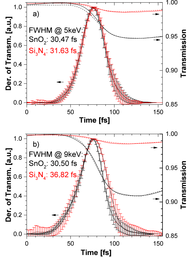
FIG. 4. a) Measured (solid lines) and calculated (dashed lines) transmission (right axis) and the derivative of the measured transmission (left axis) of \text{SnO}_2 a),b) black, \text{Si}_3\text{N}_4 a),b) red at photon energies a) 5 keV and b) 9 keV.
