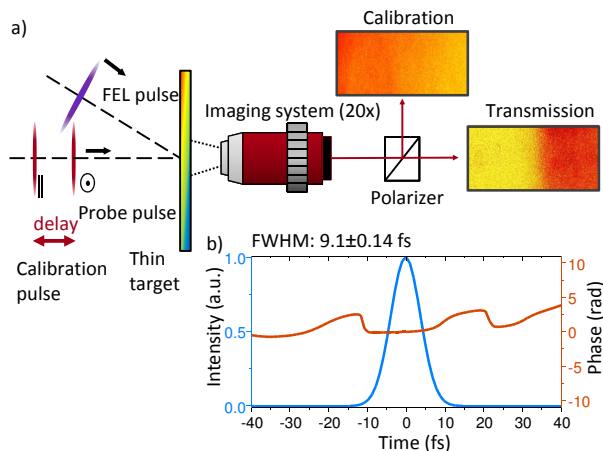
FIG. 2. a) Schematic of the experimental setup for single-shot measurement of the electron cascading processes. The FEL pulse arriving at an angle of 30° with respect to the target normal causes a fast ionization process, which is probed by an ultrashort (< 10 fs) long laser pulse at 800 nm wavelength at normal incidence. Different fractions of the X-ray wavefront are absorbed at different spatial positions on the sample, resulting in a spatio-temporal encoding of the ionization process. The first optical pulse probes the ionization process and then the outcome is recorded in the transmission measurement image. The surface of the thin target is imaged onto two CCD cameras separated by a broadband polarizer cube. b) Reconstructed temporal intensity and phase profile of the probe pulse from single shot FROG trace, FWHM = 9.1 ± 0.14 fs
