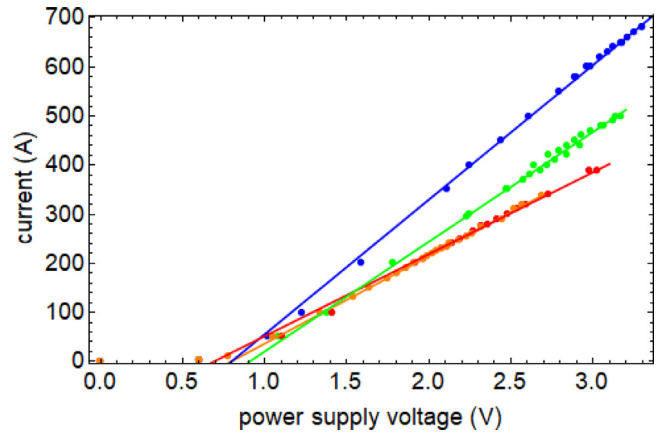
Fig. 18. The measured supply voltage and output current show the IGBT threshold and the series resistance for octupole (blue), quadrupole (green), pinch (red) and bucking (orange) coil circuits. (For interpretation of the references to color in this figure legend, the reader is referred to the web version of this article.)
