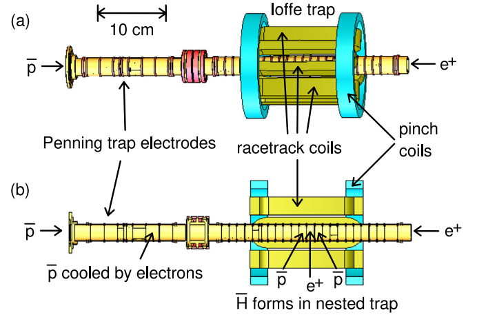
Fig. 3. A scale representation of the ATRAP first generation Penning-Ioffe trap. There is a spatially uniform magnetic field directed parallel to the trap axis that is produced by an external solenoid (not shown).
