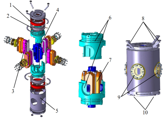
Fig. 4. Exploded view of the first generation Ioffe trap. Colors are used to distinguish components rather than signify material. The labeled parts are: 1. pinch coil; 2. winding form for pinch coil; 3. racetrack coil for quadrupole field; 4. winding form for racetrack coils (aluminum); 5. titanium vacuum vessel; 6. aluminum clamps for coil support; 7. aluminum rings for racetrack coil support; 8. connection ports, two for coil leads and one for an unobstructed path for boiled-off He gas; 9. radial access sideports; and 10. ports for LHe connection to the field-boosting solenoid mounted below the Ioffe trap. (For interpretation of the references to color in this figure legend, the reader is referred to the web version of this article.)
