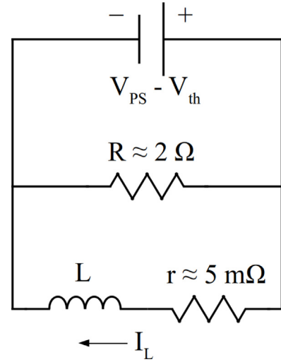
Fig. 17. The effective circuit for charging each Ioffe coil.
