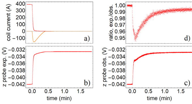
Fig. 22. Comparison of expected and measured Hall probe data during a fast dump of the pinch coil: (a) The measured currents in the pinch (red) and bucking (orange) coils (b) The z -probe response we would expect from these currents (c) The measured z -probe voltages (d) The ratio of the expected voltages to the measured voltages. (For interpretation of the references to color in this figure legend, the reader is referred to the web version of this article.)
