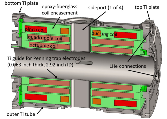
Fig. 6. Scale cross section of the Ioffe trap and its enclosure, with major components and features annotated.
