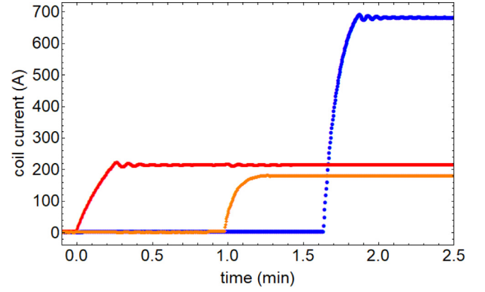
Fig. 21. Coil currents during the automated ramp-up routine for a full-depth octupole trap, with the octupole current (680 A) in blue, the pinch current (210 A) in red, and the bucking current (179 A) in orange. (For interpretation of the references to color in this figure legend, the reader is referred to the web version of this article.)
