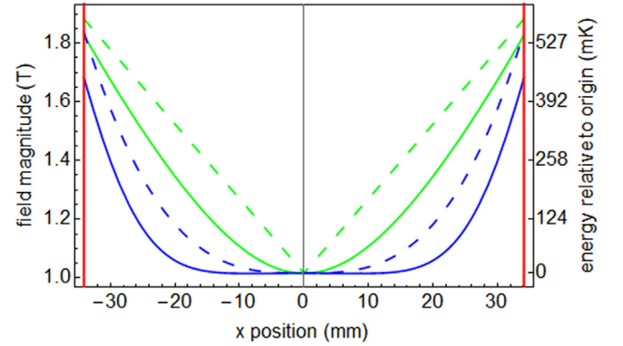
Fig. 9. The field magnitude and potential energy at z = 0 for an \bar{H} atom near the center of the ATRAP quadrupole (green) and octupole (blue) Penning-Ioffe traps with a 1 T bias field. Dashed curves are |x| and |x|^3 dependencies for comparison. The red lines are at the inner radius of the Penning trap electrodes. (For interpretation of the references to color in this figure legend, the reader is referred to the web version of this article.)
