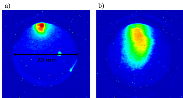
Fig. 30. (a) An example image of a positron plasma, with the 20 mm diameter of the visible surface of the phosphor screen indicated. The movable stage the imaging system was mounted to did not have sufficient range of motion to center the imaging system on the trap axis. (b) An example image of a less-compressed antiproton plasma.
