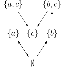
(b) CS derived from \mathcal{E}
