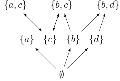
(b) The CS derived from \mathcal{E}
