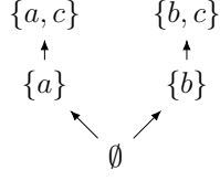
Figure 5: Domain corresponding to SES \mathcal{E} of Example 2.29.
