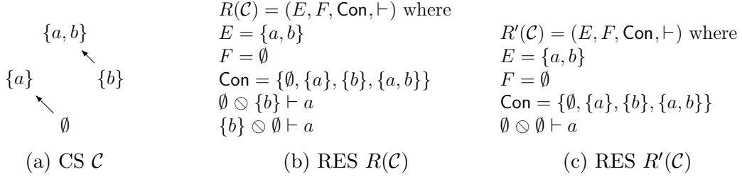
Figure 17: Example of a CS and the two different corresponding RESs.
