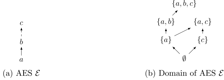
Figure 4: Example of an AES and the corresponding domain.
