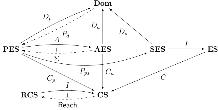
Figure 8: Categories of forward-only event structures and CSs. We use dashed lines to indicate functors which do not commute with the rest of the diagram.
