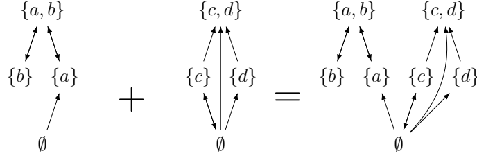
Figure 6: Example of a coproduct
