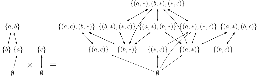
Figure 7: Example of a Product
