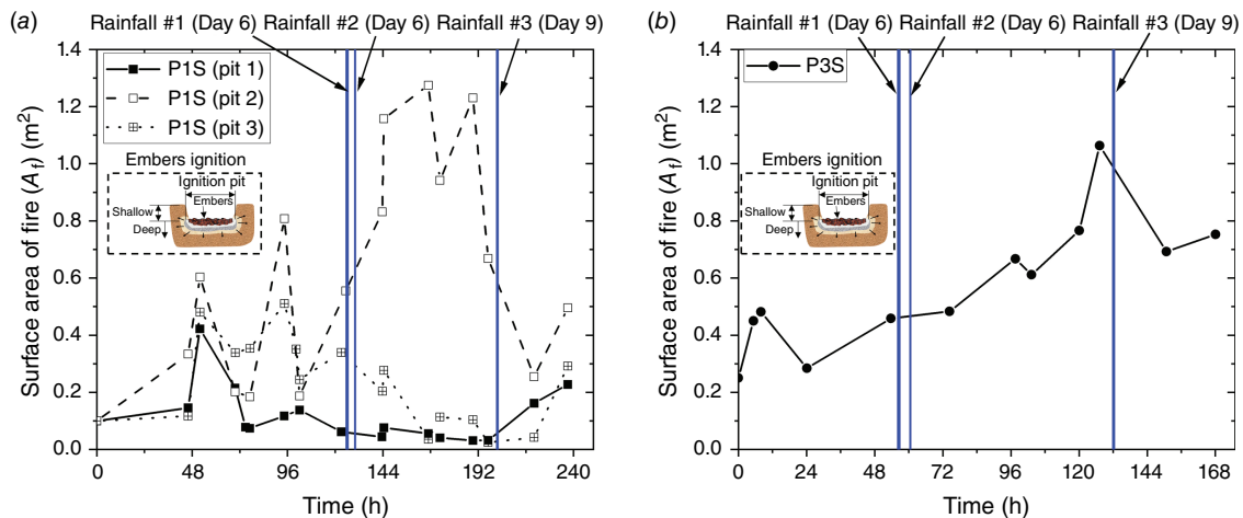
Fig. 10. Surface area of smouldering fires in (a) P1S and (b) P3S measured by infrared imaging. The x-axis time of P1S and P3S are different. Time at 0 h in each plot represents their time of ignition. The last data point represents measurement before controlled suppression on Day 11.
