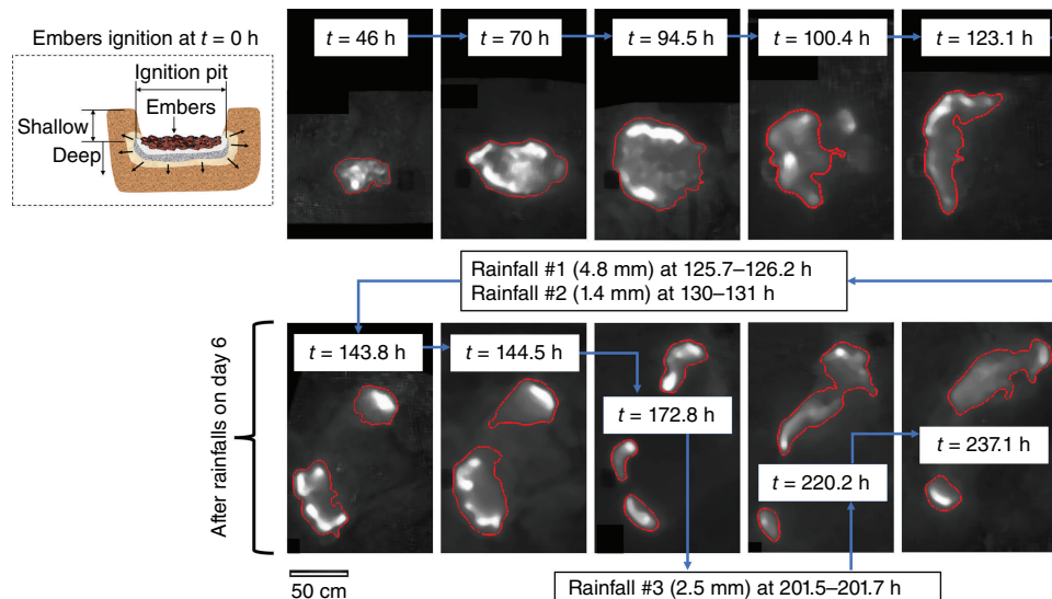
Fig. 11. Evolution of a smouldering hotspot at the surface as measured by infrared camera on Pit 3 of P1S from t = 46 to 237.1 h. Time at 0 h is the time of ignition. Rainfalls occurred at t = 125.7 , t = 130 and t = 201.5 h. The suppression of this fire was at t \sim 244 h.
