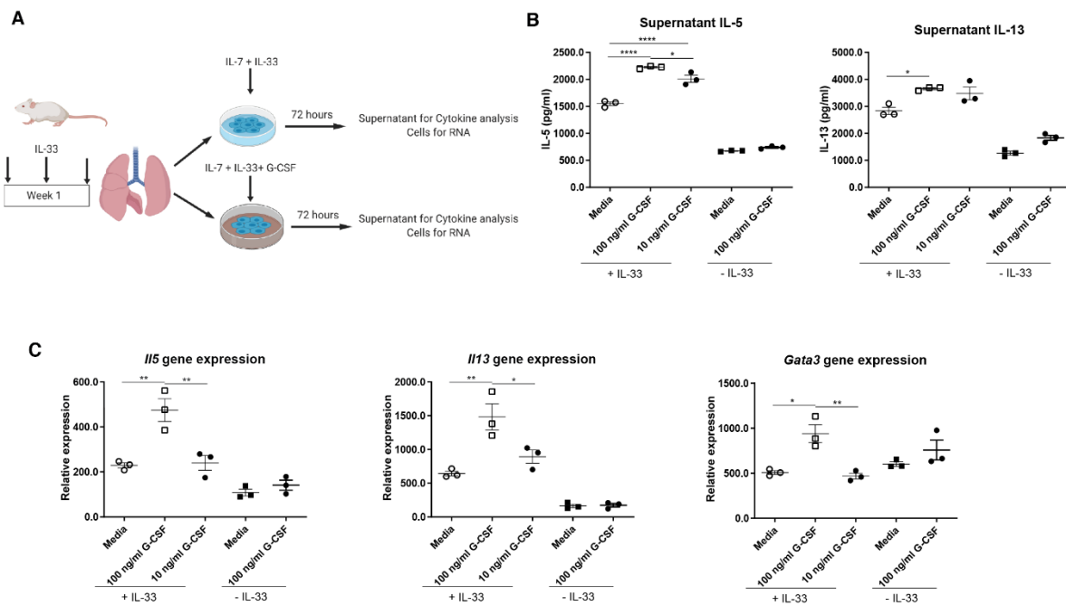
Supplementary Fig. 17: G-CSF directly augments TH2 cytokine production from mouse ILC2s.
