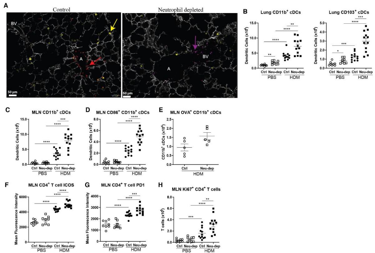
Supplementary Fig. 12: HDM exposed, neutrophil depleted mice exhibit augmented dendritic cell numbers and antigen presentation.
