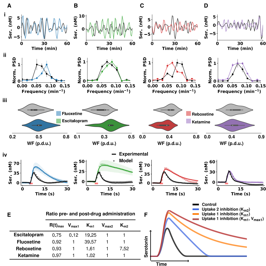
Figure 2. Serotonergic oscillations from ambient measurements and FSCV responses
