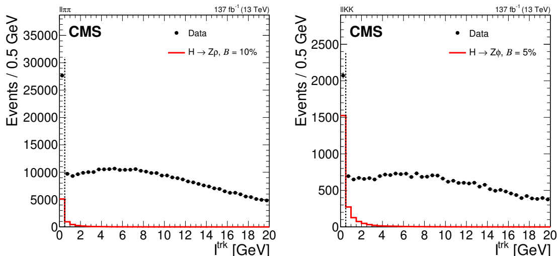
Figure 4. The ditrack isolation sum in the \ell\ell\pi\pi (left) and \ell\ell KK (right) channels, combining the \mu\mu and ee channels for all the data-taking years. The distribution in data, as well as in the simulated H \rightarrow Z\rho and H \rightarrow Z\phi signals is shown. A branching fraction of 10 (5)% for the H \rightarrow Z\rho ( H \rightarrow Z\phi ) signal is assumed. The isolation sum is shown after applying all selection criteria apart from the ditrack isolation requirement. The ditrack invariant mass requirement is also applied. Only events in which the dilepton plus ditrack invariant mass is in the range 120–130 GeV are considered. The dashed line indicates the boundary of the region used in the analysis, for which the isolation sum is required to be smaller than 0.5 GeV.
