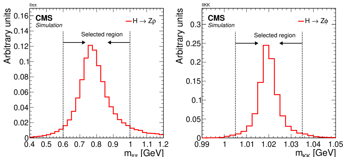
Figure 5. Distribution of the ditrack invariant mass in simulated H \rightarrow Z\rho events passing the \ell\ell\pi\pi selection criteria (left) and in simulated H \rightarrow Z\phi events passing the \ell\ell KK selection criteria (right). These masses are calculated assuming the charged particle mass equals the pion mass in the \ell\ell\pi\pi selection and assuming the charged particle mass equals the kaon mass in the \ell\ell KK selection. The events pass all selection criteria described in the text, apart from the requirements on the ditrack invariant mass window. The dashed lines indicate the region selected in the analysis.
