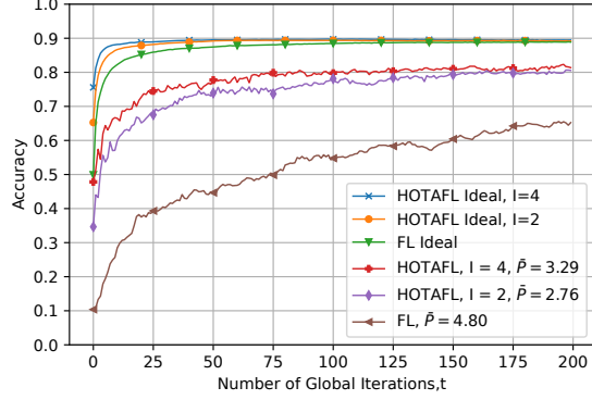
Fig. 3: Test accuracy for non-i.i.d. MNIST data with \tau = 3 .
