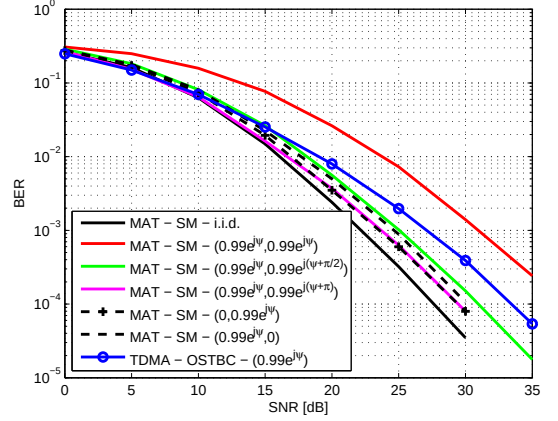
Fig. 4. Average Bit Error Rate (BER) of SM-encoded MAT (with R=4/3 bit/s/Hz per user) over spatially correlated channels (t_1, t_2) . Phase \psi is random and uniformly distributed within [0, 2\pi] . Comparison with TDMA - OSTBC ( R=3/2 bit/s/Hz) is also provided.
