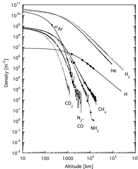
Figure 2: Density profiles in the lunar exosphere for volatile species on the dayside (at a surface temperature of 400K) based on measurements or upper limits (Heiken et al., 1991; Stern, 1999; Killen and Ip, 1999). Figure is from Wurz et al. (2012).
