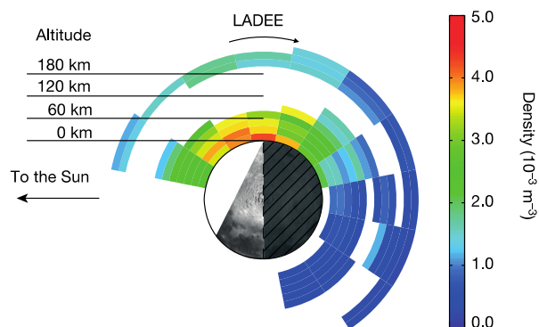
Figure 4: The top-down view of the dust particle density ( a > 0.3 \mu\text{m} ) projected onto the lunar equatorial plane. While pointed near the direction of the motion of the spacecraft, LDEX did not make measurements between 12 and 18 local time. White coloring indicates regions where LADEE did not visit or was not set up for normal operations. Figure is from Horányi et al. (2015).
