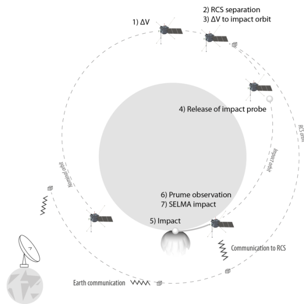
Figure 5: Impact experiment sequence to investigate a permanently shadowed region (not in scale).
