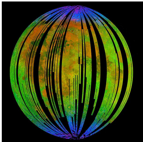
Figure 1: Three-color composite image of reflected near-infrared radiation from the Sun as obtained by M3. Blue shows the signature of water and hydroxyl molecules as seen by a highly diagnostic absorption of infrared light with a wavelength of 3 \mu m. Green shows the brightness of the surface as measured by reflected infrared radiation from the Sun with a wavelength of 2.4- \mu m, and red shows an iron-bearing mineral called pyroxene, detected by absorption of infrared light at 2.0- \mu m. The figure is from Pieters et al. (2009) .
