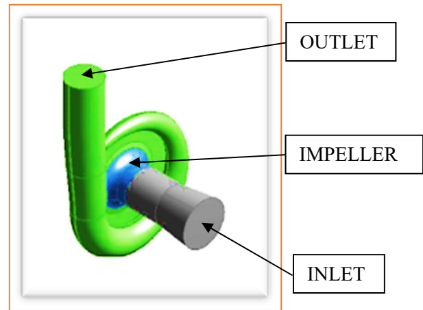
Figure 1 Fluid Domain
