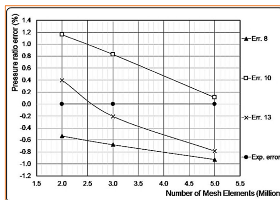
Figure 9 Pressure Ratio Error at 80,000 rpm
