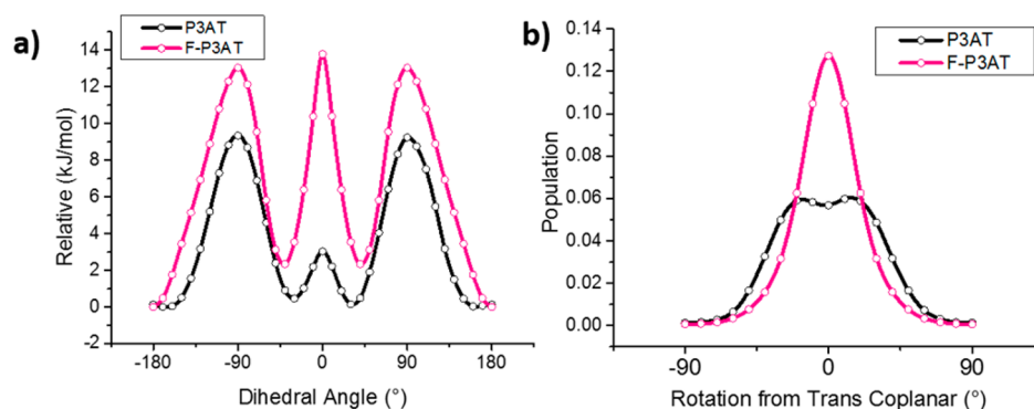
Figure 5. a) Potential energy distribution of P3AT and F-P3AT, where A = methyl. A dihedral angle of 0^\circ corresponds to the cisoid conformation; b) Relative probability densities for populating the energy distribution with a Boltzmann energy distribution at room temperature. A dihedral angle of 0^\circ corresponds to the transoid configuration.
