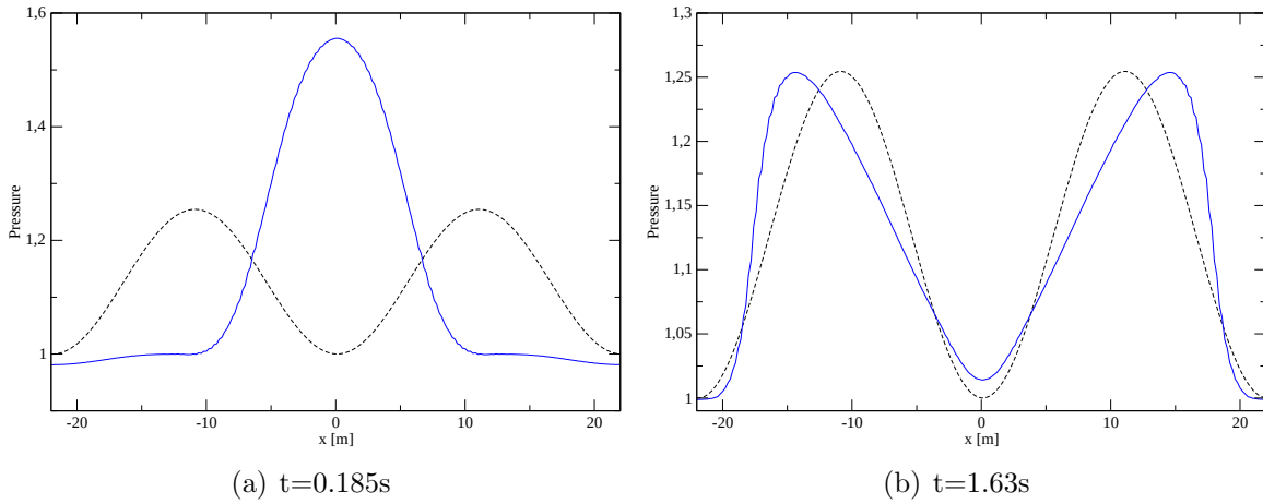
Figure 2: Pressure profiles as functions of space at a given time in the colliding pulses test-case. The initial profile is in dashed line, and the solid line provides the results of the second-order scheme at two different times.
