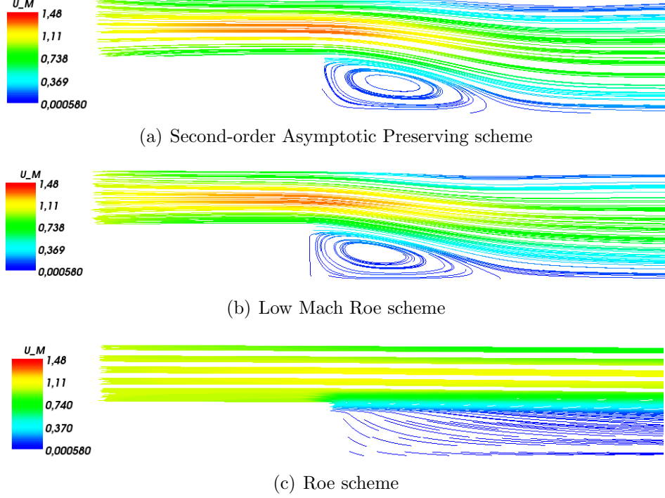
Figure 8: Backward facing step test-case for a Reynolds number \text{Re} = 75 - Streamlines
