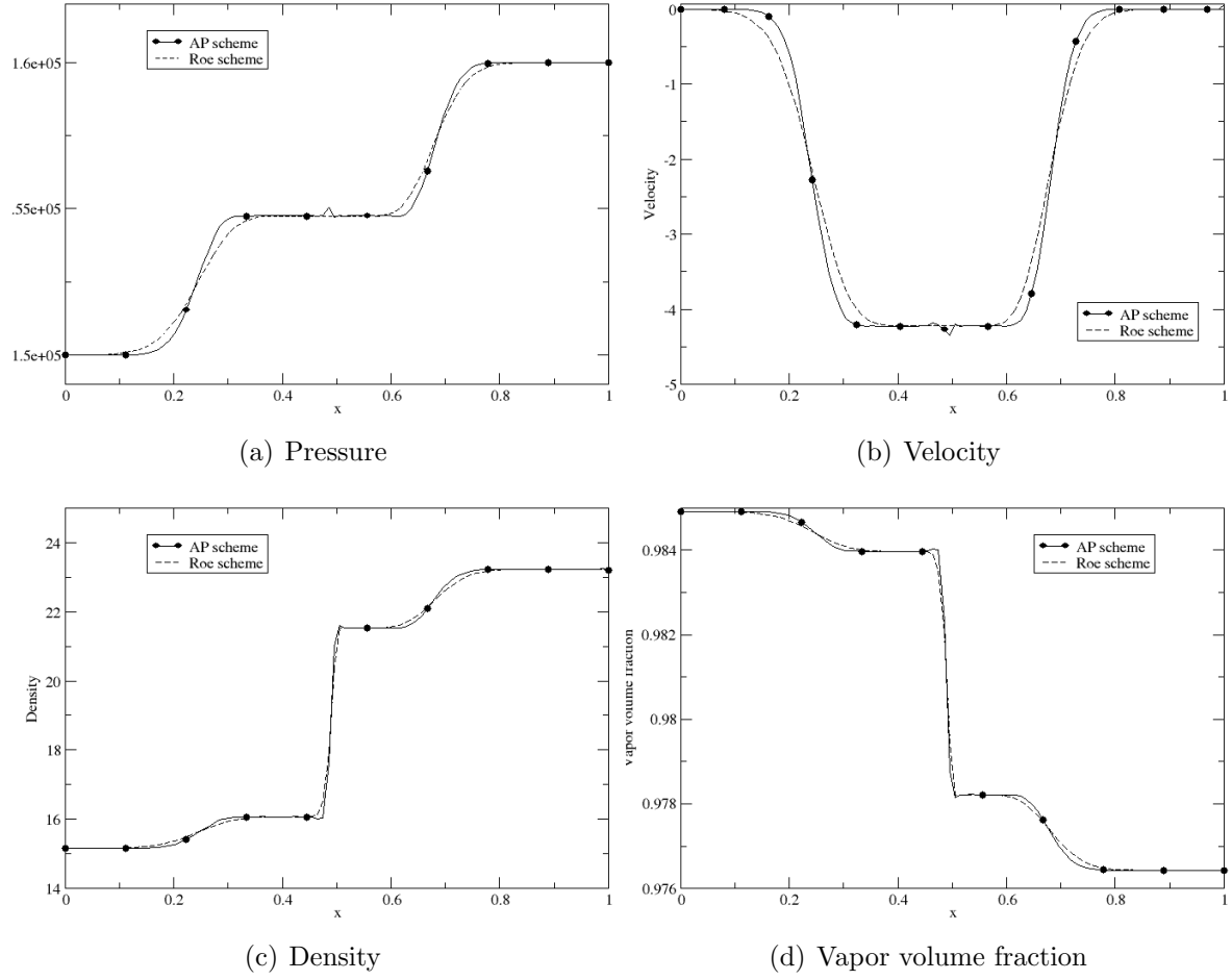
Figure 6: Two-phase flow shock tube problem. Pressure, velocity, density, and vapor volume fraction profiles as functions of space at time t = 3.5 \cdot 10^{-3} s.
