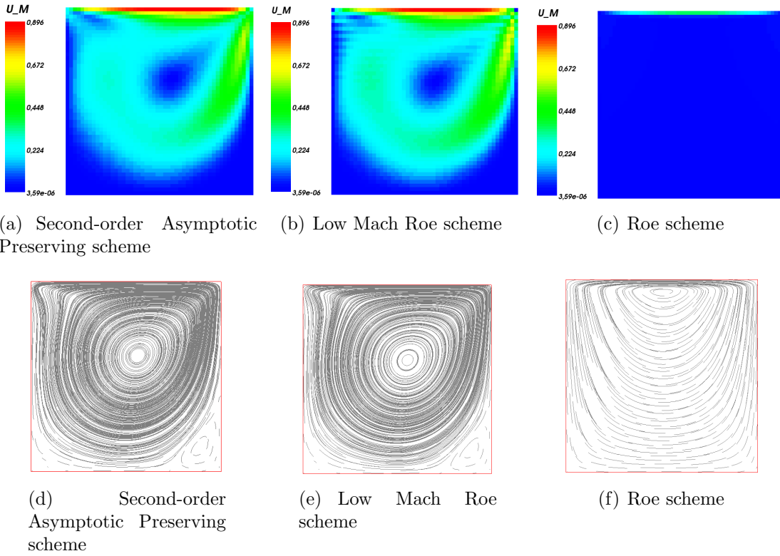
Figure 9: Lid-driven cavity test-case - Modulus of the velocity and streamlines.
