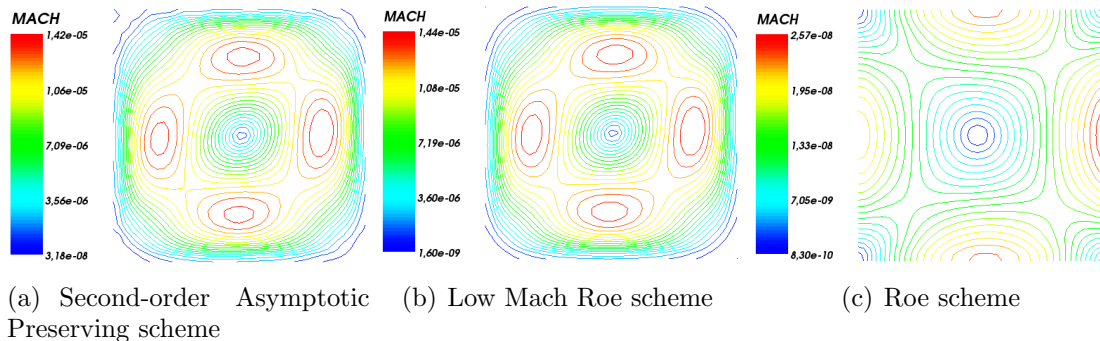
Figure 10: Heat-driven cavity test-case - Isocontours of the Mach number
