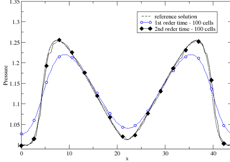
Figure 3: Colliding pulses test-case: pressure profiles as a function of space at a given time. Comparison of first and second order in time schemes with a reference solution. The solution obtained with the second order-in-time scheme is very close to the reference solution.
