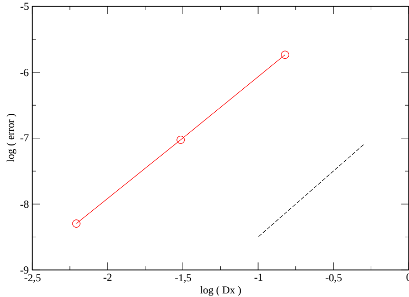
Figure 4: Convergence test for the second order in time and space scheme, with \alpha = \frac{1}{\epsilon^2} . The solid line gives the L^1 error as a function of \Delta x in log-log scale. The dashed line displays a straight line of slope equal to 2 for the sake of comparison.
