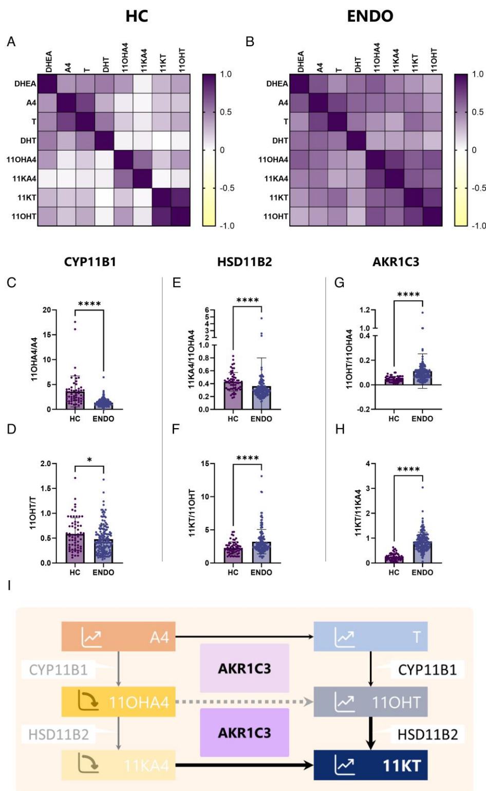
Figure 2. Endometriosis is associated with altered androgen metabolism characterized by increased production of 11KT. (A) Pearson correlation matrix of key analytes in HC demonstrates strong correlation between related steroids within relevant subgroups including A4 and T, 11OHA4 and 11KA4 as well as 11KT and 11OHT. (B) In patients with ENDO, there was a strong correlation between both classic and 11-oxygenated androgen metabolites indicative of altered metabolism. Enzyme activity based on substrate to product ratios (product/substrate) were calculated based on measured serum concentrations in healthy control women (HC) and patients diagnosed with endometriosis (ENDO). The ratios required for sequential production of 11KT were assessed including CYP11B1 (C, D), HSD11B2 (E, F), and AKR1C3 (G, H). The ratios of 11OHA4/A4 (C), 11OHT/T (D), and 11KA4/11OHA4 (E) were significantly decreased in ENDO compared with HC. In contrast, the ratios of 11KT/11OHT (F), 11OHT/11OHA4 (G), and 11KT/11KA4 (H) were significantly increased in ENDO compared with HC. Collectively, these metabolism changes are associated with increased production of 11KT (I). Statistical comparison using Mann-Whitney U test. * P <0.05, **** P <0.0001.
