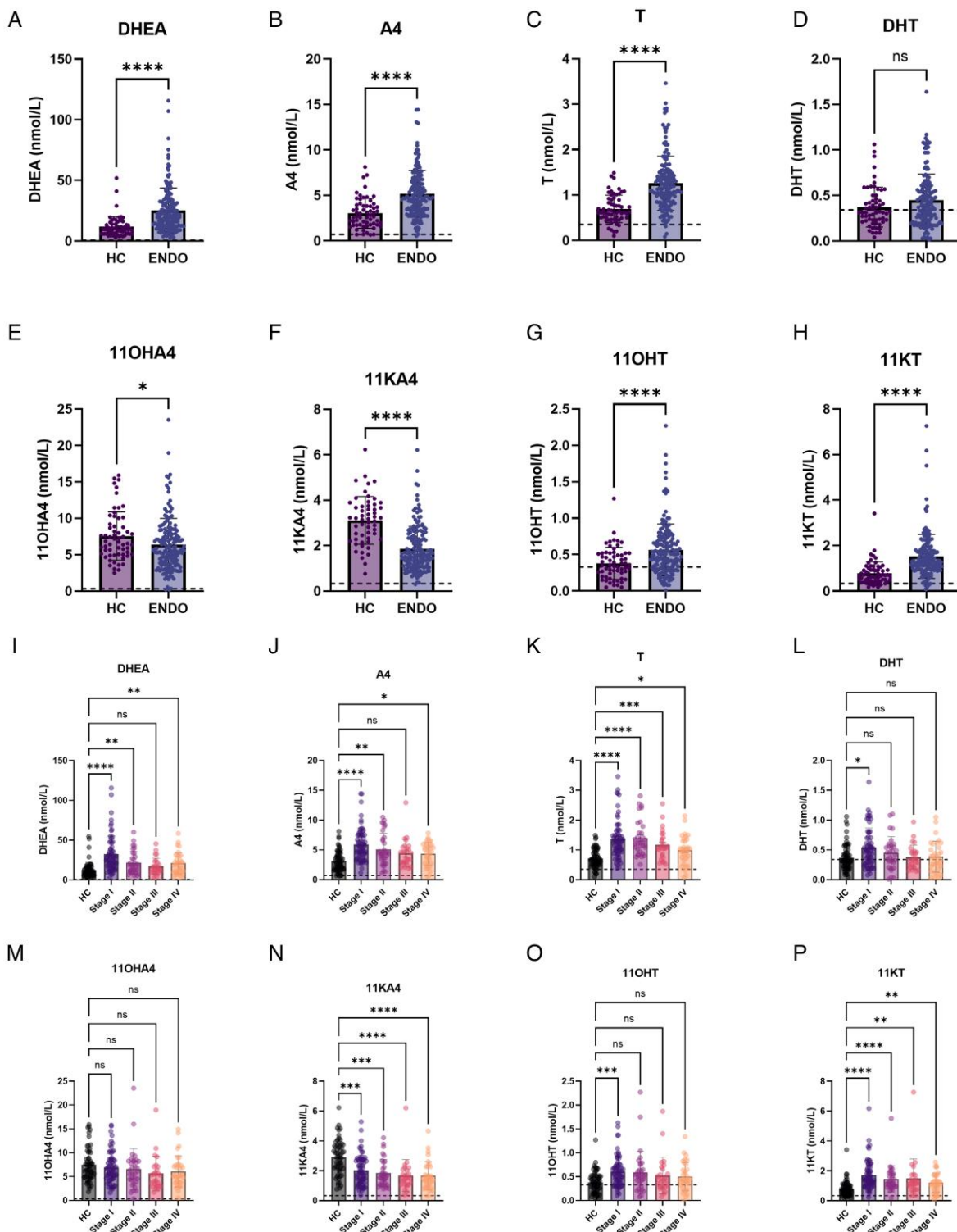
Figure 1. Serum concentrations of classic and 11-oxygenated androgens are altered in women with endometriosis. Serum concentrations of DHEA, A4, T, 11OHA4, 11KA4, 11OHT, and 11KT were determined by LC-MS/MS. DHEA, A4, and T were significantly elevated in women with endometriosis (ENDO) compared with healthy controls (HCs; A-C). Concentrations of DHT did not differ between groups (D). 11-oxygenated androgen precursors, 11OHA4 (E) and 11KA4 (F), were decreased in ENDO, while potent 11-oxygenated androgens, 11OHT (G) and 11KT (H) were significantly elevated in ENDO. Patients with ENDO were stratified according to rASRM stage (I-P). DHEA and A4 were significantly elevated in Stage I, II, and IV endometriosis (I, J). T was elevated in all endometriosis stages (K), and DHT was significantly elevated in Stage I endometriosis (L). Concentrations of 11OHA4 did not significantly differ between groups (M) while 11KA4 was decreased in all stages (N). In contrast, 11OHT was significantly elevated in Stage I endometriosis (O) while 11KT was elevated in all endometriosis stages (P). Median serum steroid concentrations (25th-75th centile range; nmol/L) for each stage (I). Error bars represent the SD of the mean. Dotted lines denote LLOQ for each analyte. Undetected steroids or those detected below LLOQ were replaced by 0.5 \times \text{LLOQ} for statistical purposes. Statistical comparison using Mann-Whitney U test or Kruskal-Wallis test with multiple comparisons. * P < 0.05 , ** P < 0.01 , *** P < 0.001 , **** P < 0.0001 . ns, non-significant.
