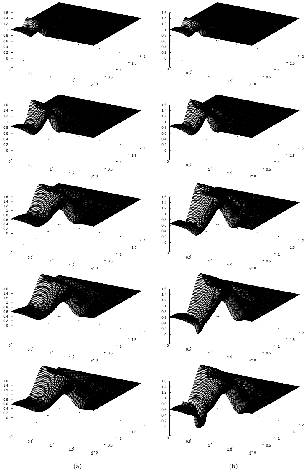
FIG. 7. U_\varepsilon(x, t_n) plotted against x at times t_n = 0.01, 0.1, 0.5, 0.7, 0.8 ; (a) without and (b) with van der Waals forces being present.
