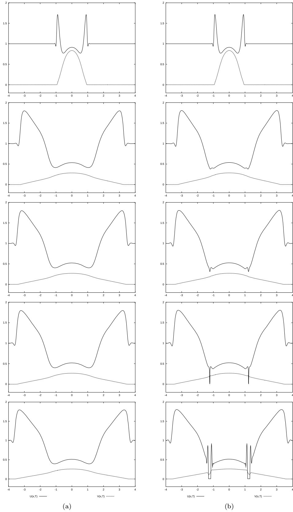
FIG. 4. U_\varepsilon(x, t_n) and V_\varepsilon(x, t_n) plotted against x at times t_n = 0.1, 6.0, 7.0, 7.3, 8.0 ; (a) without and (b) with van der Waals forces being present.
