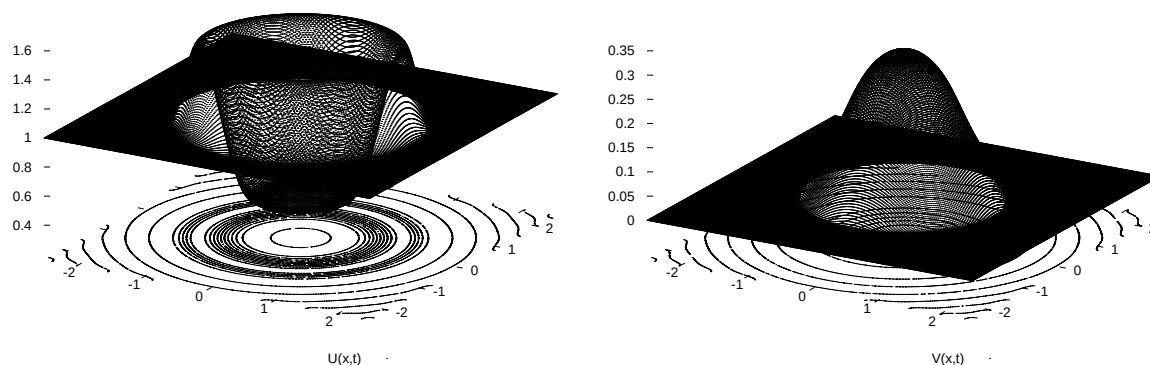
FIG. 8. U_\varepsilon(x, T) and V_\varepsilon(x, T) plotted against x for T = 1 .
