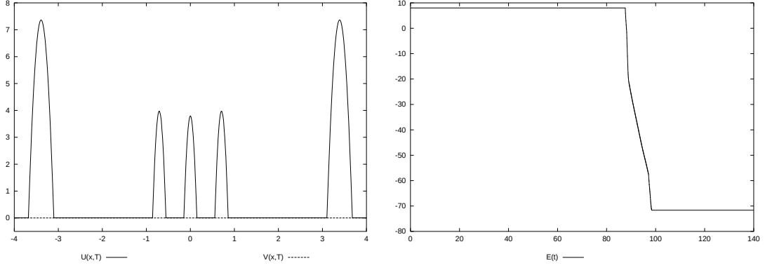
FIG. 1. U_\varepsilon(x, T) and V_\varepsilon(x, T) plotted against x at T = 140 and E(t) for t \in [0, T] .
