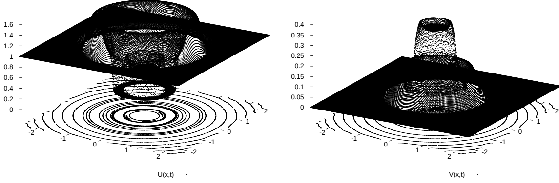
FIG. 5. U_\varepsilon(x, T) and V_\varepsilon(x, T) plotted against x for T = 1 .
