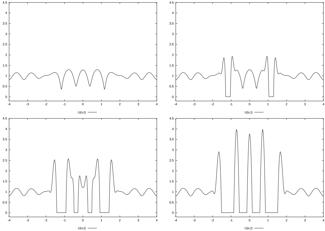
FIG. 2. U_\varepsilon(x, t) plotted against x at t = 87.5, 88, 88.5, 89 .
