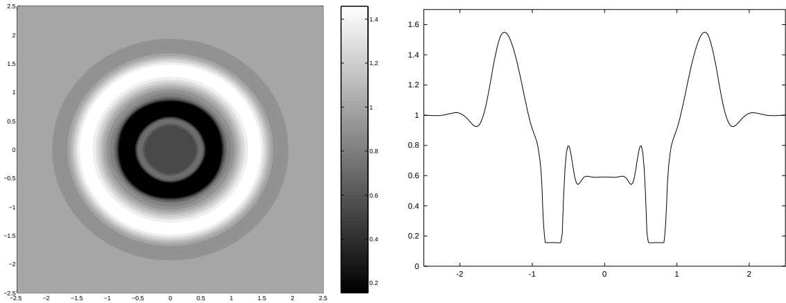
FIG. 6. Contour plot of U_\varepsilon(x, T) and U_\varepsilon(x, T)|_{x_2=0} plotted against x_1 for T = 1 .
