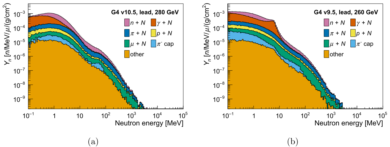
Fig. 4 Energy spectra of neutrons produced in lead from different production processes. Production spectra a from 280 GeV muons were simulated with GEANT4 version 10.5 and b from 260 GeV muons were simulated with version 9.5. The dominant processes are described in the caption of Fig. 3
