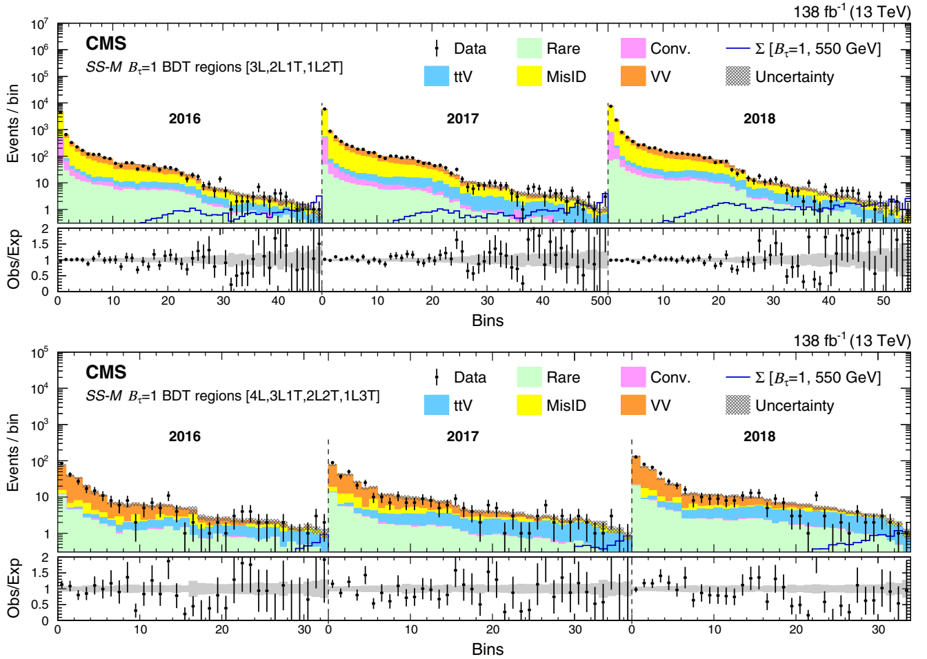
FIG. 16. The SS\text{-}M B_\tau = 1 BDT regions for the 3-lepton (upper) and 4-lepton (lower) channels for the 2016–2018 datasets. The lower panel shows the ratio of observed events to the total expected background prediction. The gray band on the ratio represents the sum of statistical and systematic uncertainties in the SM background prediction. The expected SM background distributions and the uncertainties are shown after fitting the data under the background-only hypothesis. For illustration, an example signal hypothesis for the production of the type-III seesaw heavy fermions in the scenario with mixing exclusively to \tau lepton for m_\Sigma = 550 GeV, before the fit, is also overlaid.
