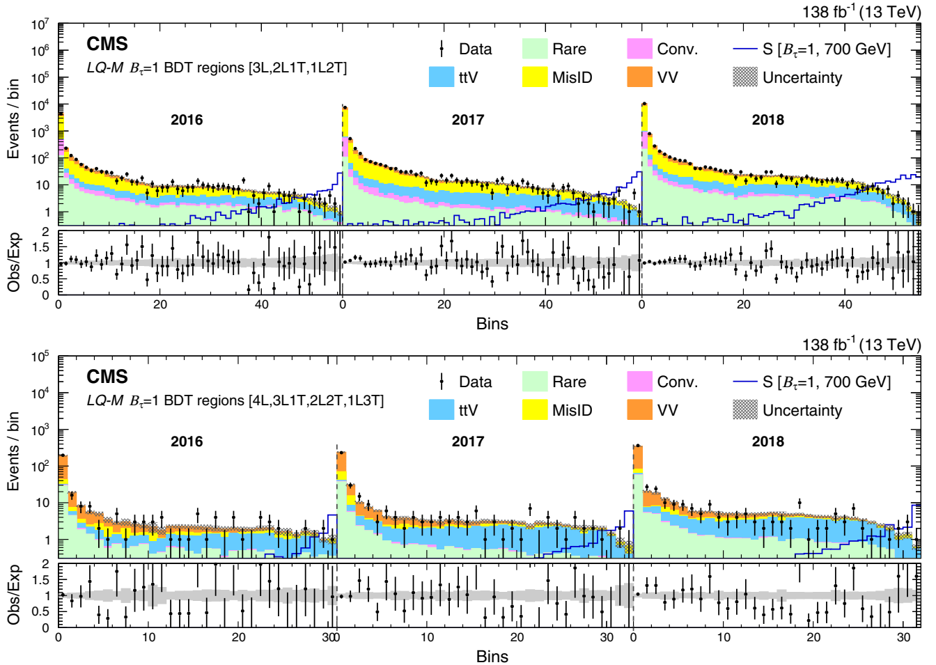
FIG. 20. The LQ\text{-}M B_\tau = 1 BDT regions for the 3-lepton (upper) and 4-lepton (lower) channels for the 2016–2018 datasets. The lower panel shows the ratio of observed events to the total expected background prediction. The gray band on the ratio represents the sum of statistical and systematic uncertainties in the SM background prediction. The expected SM background distributions and the uncertainties are shown after fitting the data under the background-only hypothesis. For illustration, an example signal hypothesis for the production of the scalar leptoquark coupled to a top quark and a \tau lepton for m_S = 700 GeV, before the fit, is also overlaid.
