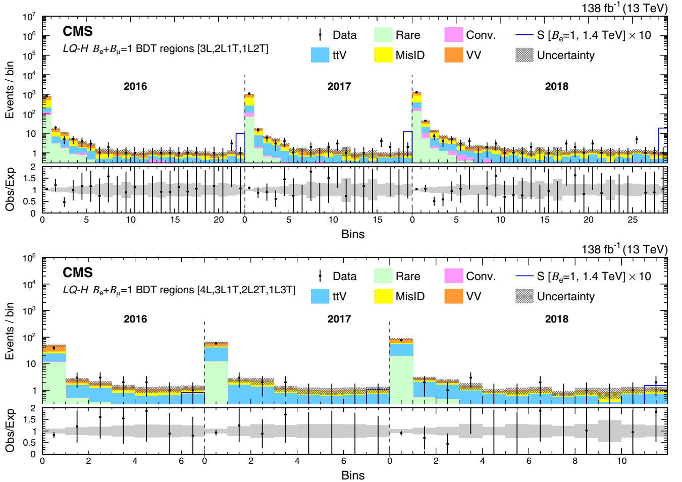
FIG. 23. The LQ\text{-}H B_e + B_\mu = 1 BDT regions for the 3-lepton (upper) and 4-lepton (lower) channels for the 2016–2018 datasets. The lower panel shows the ratio of observed events to the total expected background prediction. The gray band on the ratio represents the sum of statistical and systematic uncertainties in the SM background prediction. The expected SM background distributions and the uncertainties are shown after fitting the data under the background-only hypothesis. For illustration, an example signal hypothesis for the production of the scalar leptoquark coupled to a top quark and an electron for m_S = 1.4 TeV, before the fit, is also overlaid.
