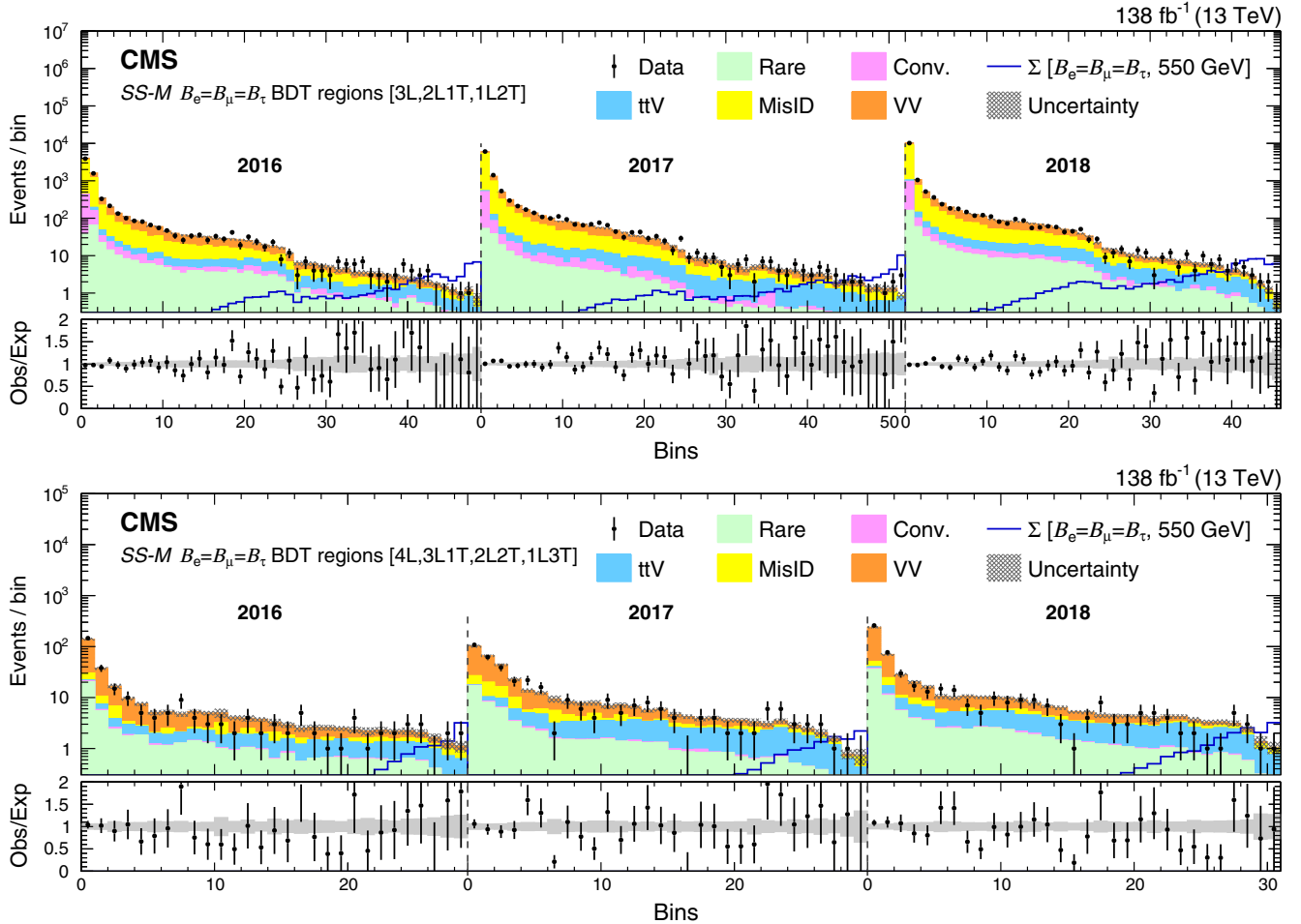
FIG. 14. The SS\text{-}M B_e = B_\mu = B_\tau BDT regions for the 3-lepton (upper) and 4-lepton (lower) channels for the 2016–2018 datasets. The lower panel shows the ratio of observed events to the total expected background prediction. The gray band on the ratio represents the sum of statistical and systematic uncertainties in the SM background prediction. The expected SM background distributions and the uncertainties are shown after fitting the data under the background-only hypothesis. For illustration, an example signal hypothesis for the production of the type-III seesaw heavy fermions in the flavor-democratic scenario for m_\Sigma = 550 GeV, before the fit, is also overlaid.
