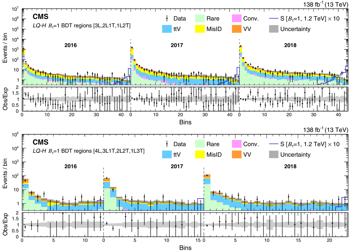
FIG. 21. The LQ\text{-}H B_\tau = 1 BDT regions for the 3-lepton (upper) and 4-lepton (lower) channels for the 2016–2018 datasets. The lower panel shows the ratio of observed events to the total expected background prediction. The gray band on the ratio represents the sum of statistical and systematic uncertainties in the SM background prediction. The expected SM background distributions and the uncertainties are shown after fitting the data under the background-only hypothesis. For illustration, an example signal hypothesis for the production of the scalar leptoquark coupled to a top quark and a \tau lepton for m_S = 1.2 TeV, before the fit, is also overlaid.
