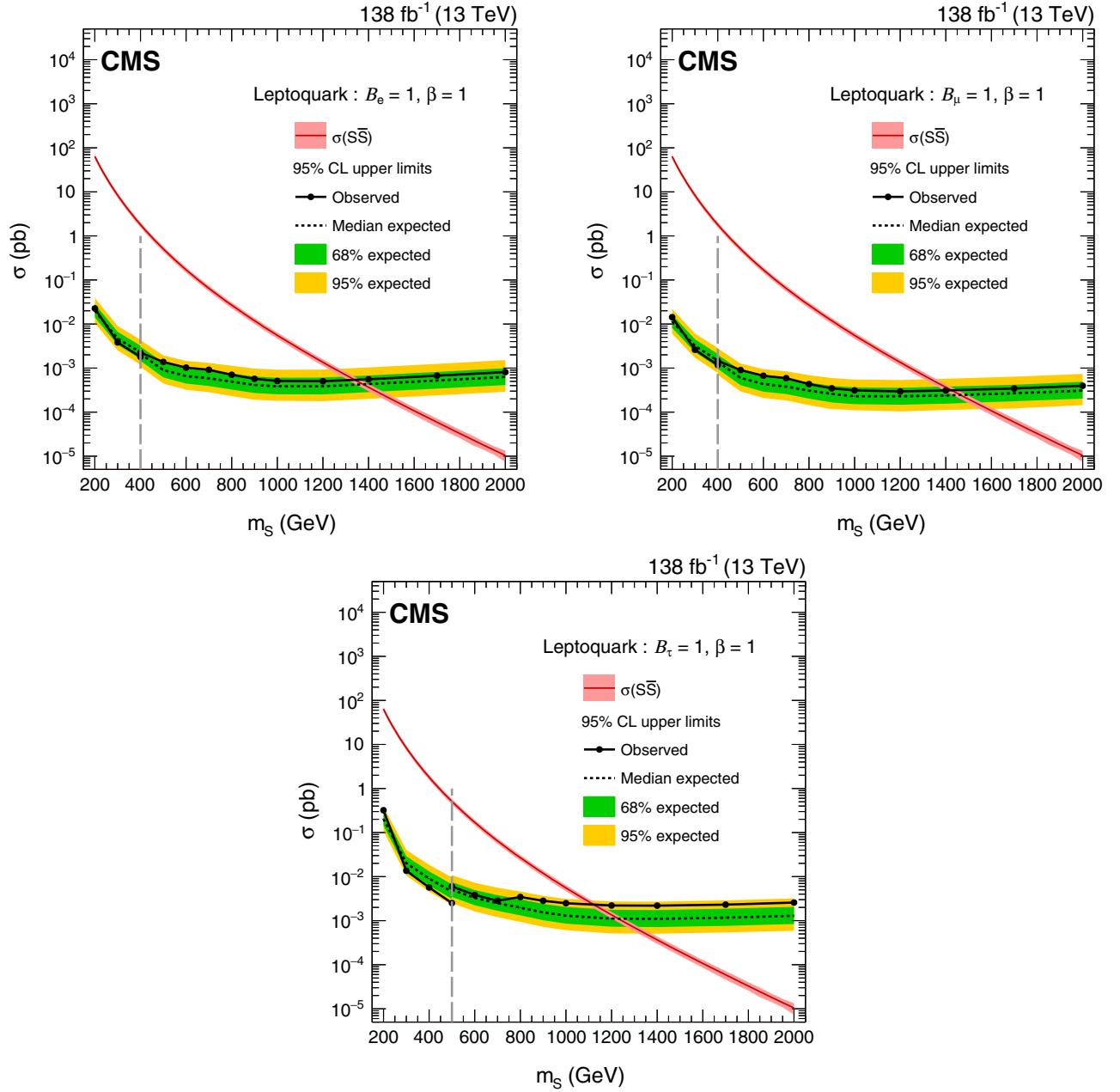
FIG. 27. Observed and expected upper limits at 95% CL on the production cross section for the scalar leptoquarks: B_e = 1 (upper left), B_\mu = 1 (upper right), and B_\tau = 1 (lower). In each figure, the limits to the left of the vertical dashed gray line are shown from the advanced S_T table, and to the right are shown from the BDT regions.
