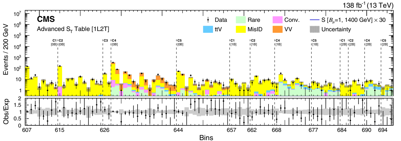
FIG. 12. The 1L2T SR distribution of the advanced S_T table for the combined 2016–2018 dataset. The detailed description of the bin numbers can be found in Table V. The lower panel shows the ratio of observed events to the total expected background prediction. The gray band on the ratio represents the sum of statistical and systematic uncertainties in the SM background prediction. The expected SM background distributions and the uncertainties are shown after fitting the data under the background-only hypothesis. An example signal hypothesis for the production of the scalar leptoquark coupled to a top quark and a muon for m_S = 1.4 TeV, before the fit, is also overlaid. For this category, the signal yield is negligible and is not visible in the figure.
