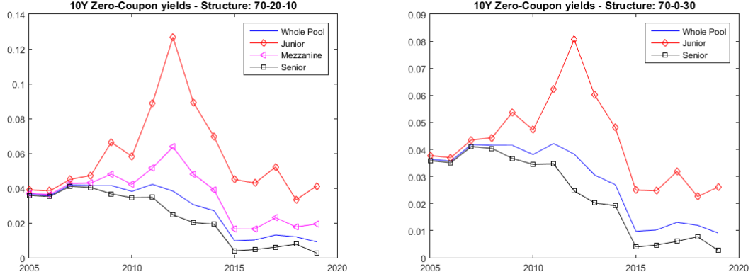
Figure 1: Time evolution of the 10Y zero coupon bonds yield rates.
