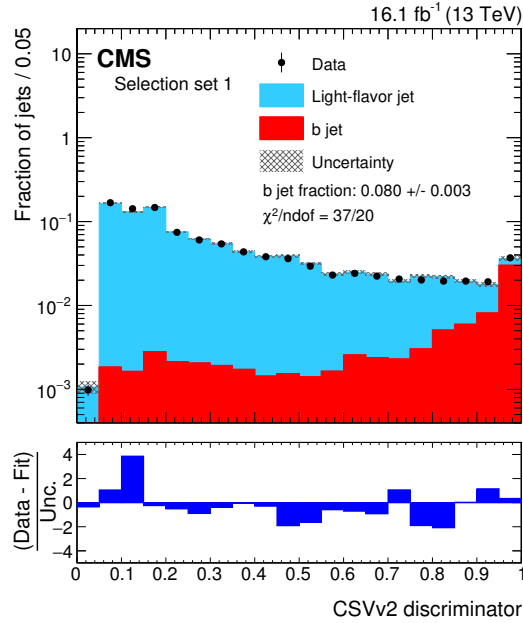
Figure 6. Determination of the b jet fraction by fitting the CSVv2 discriminator distribution. The red and blue distributions are the CSVv2 discriminator templates of b jets and light-flavor jets, respectively. The black points with uncertainty bars show the data distribution. The uncertainties in the upper panel include statistical uncertainties of the b jet and light-flavor jet templates, and the fit uncertainties, summed in quadrature. The goodness of fit is given by the \chi^2 divided by the number of degrees of freedom (ndof). The bottom panel shows the difference between data and the fit result, divided by the combination of the statistical uncertainty of data and the uncertainty from the upper panel. The distributions are derived from kinematic samples resulting from selection set 1 in table 3.
