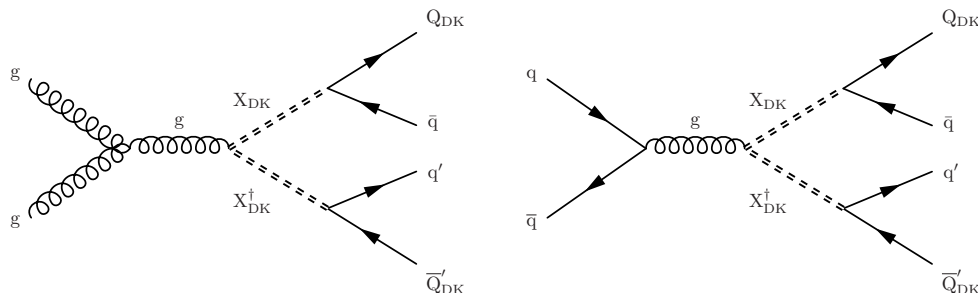
Figure 1. Feynman diagrams in the BSSW model for the pair production of mediator particles, with each mediator decaying to a quark and a dark quark Q_{DK} , via gluon-gluon fusion (left) and quark-antiquark annihilation (right).
