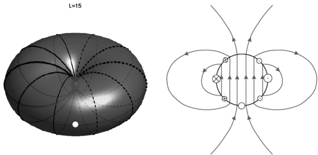
Figure 10. From Southwood and Kivelson (2007). Original caption: (left) Schematic shell of L = 15 dipolar field lines on which currents flow into and out of the northern ionosphere. If the current strength varied sinusoidally with longitude, as indicated by varying thickness of the lines representing the current, but flowed on a spherical surface, the perturbation field within the shell would be uniform. In order to produce the observed uniform field within a nonspherical surface, additional current loops must be present on the surface. (right) In a cut through the equatorial plane, field lines arising from the field-aligned currents at L = 15 shown in the left hand diagram. The field is uniform in the area inside the shell at L = 15 (here shown on a different scale) and dipolar outside of that boundary. The white dots in the two images are at the same location on the boundary.
