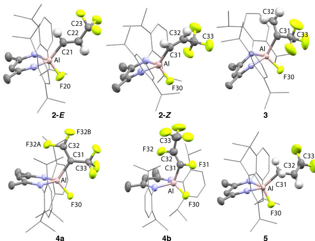
Figure 1. Solid state structures of 2-E, 2-Z, 3, 4a, 4b and 5.
