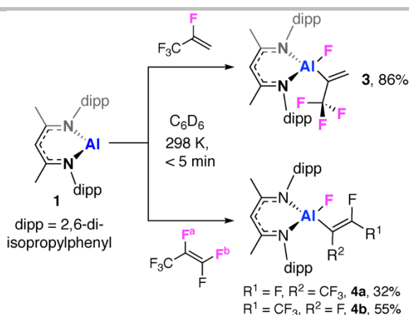
Scheme 2. Reaction of 1 with HFO-123yf and hexafluoropropene
