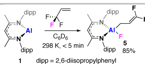
Scheme 3. Reaction of 1 with trifluoropropene
