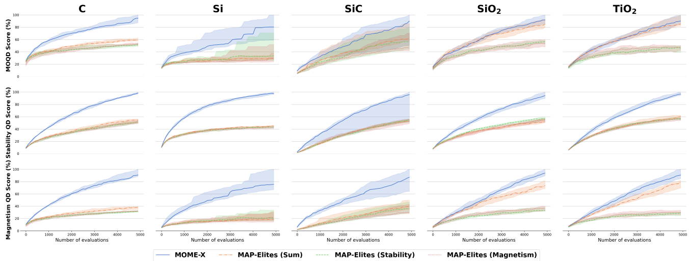
Figure 4: Median performance of 15 seeds, the shaded regions show the inter-quartile range.
