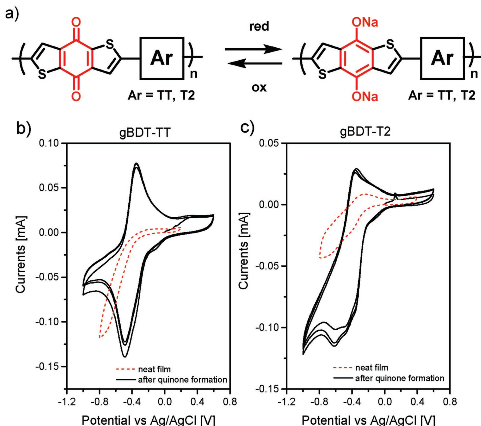
Figure 4. a) Reduction of the quinone containing copolymers to form the sodium alkoxide structure and b) CV measurements before (red dashed line) and after electrochemical oxidation (black line) of the large IP polymers with degassed 0.1 M NaCl aqueous solution.
