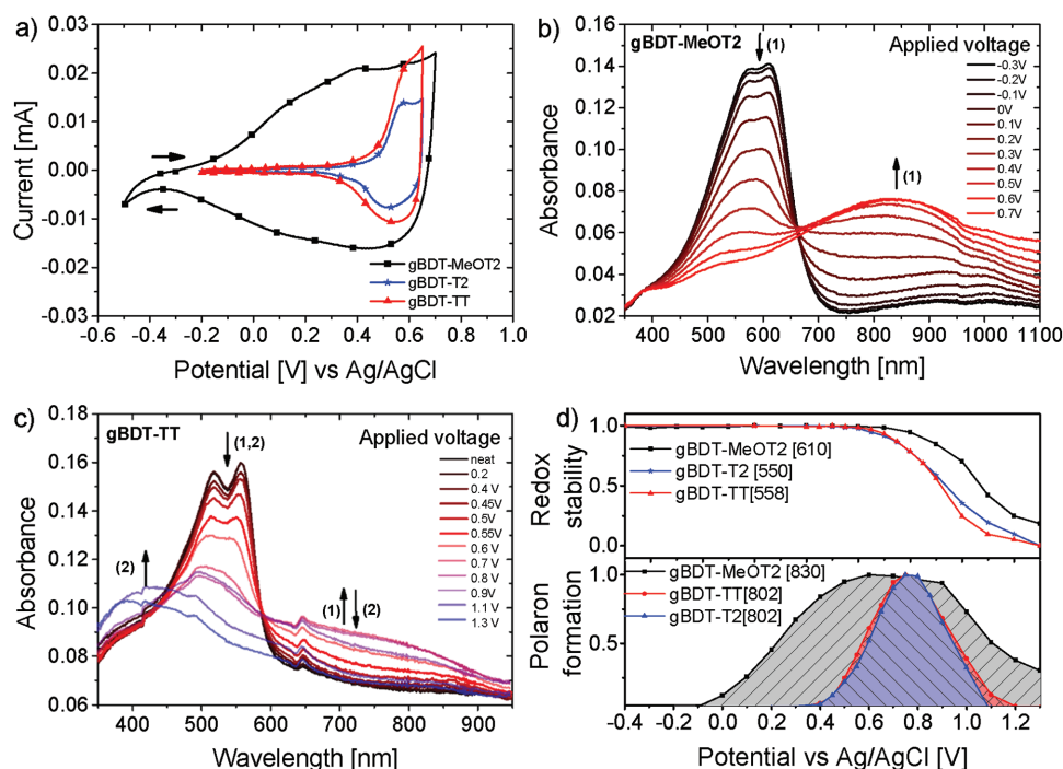
Figure 2. Electrochemical oxidation and changes in absorption. a) Cyclic voltammetry of polymer thin films with a scan rate of 100 \text{ mV s}^{-1} , b) spectroelectrochemical measurements of gBDT-MeOT2, c) spectroelectrochemical measurements of gBDT-TT ((1) formation of polaron and (2) decomposition), and d) comparison of the redox stability of the polymers after applying the indicated voltages and reversing the voltage to reduce the copolymer (top, redox stability of the copolymers (at the indicated wavelength) showing the difference of absorbance of the pristine copolymer (at -0.3 \text{ V} ) and oxidized copolymer (indicated voltage, then reversing the voltage to -0.3 \text{ V} , normalized to the maximum value) and formation of the polaron at the indicated wavelengths (bottom, normalized polaron absorbance ( \lambda_{\text{max}} (polaron)) at the indicated wavelength, area underneath the curves are highlighted, note that the area underneath the curves does not represent the amount of introduced charges). The measurements were carried out in degassed 0.1 \text{ M NaCl} aqueous solution.
