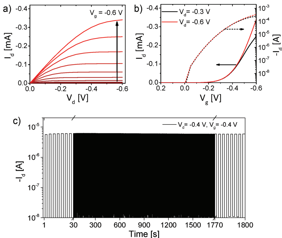
Figure 6. OECT performance of gBDT-MeOT2 with a) output curve for -0.6 \text{ V} < V_g < 0 \text{ V} ( \Delta V_g = 0.05 \text{ V} ), b) transfer curve at V_d = -0.3 and -0.6 \text{ V} for device dimensions of W = 100 \mu\text{m} , L = 10 \mu\text{m} , and d = 124 \text{ nm} and c) stability measurement of the OECT for 30 min with V_d = -0.4 \text{ V} and applying voltage pulses between V_g = 0 and -0.4 \text{ V} (the beginning and end of the pulse experiment is highlighted (30 s)).
