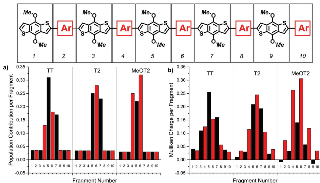
Figure 5. DFT calculations. a) Singly unoccupied molecular orbital (SUMO) and b) charge distribution in polymers gBDT-TT, gBDT-T2, and gBDT-MeOT2 bearing a positive charge, calculated at tuned- \omega B97XD/6-31G*. Each vertical bar represents the contribution from different fragments along the polymer chain (BDT in black, thiophene comonomer in red).
