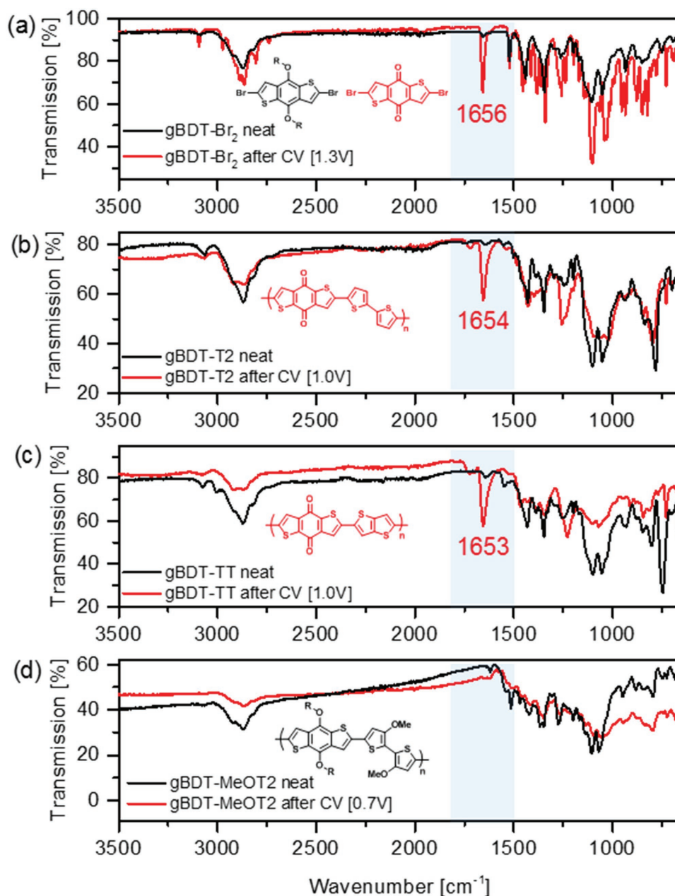
Figure 3. IR spectra and analysis of the decomposition products. a) Quinone formation of the monomer gBDT-Br 2 after applying 1.3 V (Figure S27, Supporting Information), b,c) quinone formation of the polymers gBDT-TT and gBDT-T2 after applying 1.0 V, and d) stable redox-reaction for gBDT-MeOT2 and no evidence of quinone formation after applying 0.7 V (polaron formation). The corresponding CV measurements are presented in Figures S23–S25 in the Supporting Information. Quinone formation of gBDT-MeOT2 can be observed after applying up to 1.5 V (Figure S26, Supporting Information).
