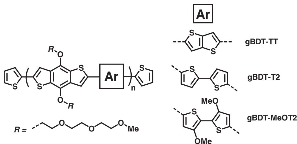
Figure 1. Chemical structures of BDT polymers gBDT-TT, gBDT-T2, and gBDT-MeOT2.
