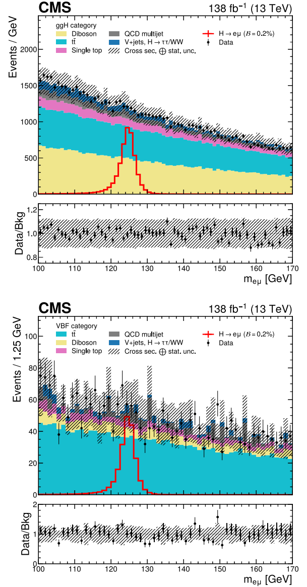
FIG. 1. The m_{e\mu} distributions of the data, simulated backgrounds and signals of H \rightarrow e\mu in the ggH (upper) and the VBF (lower) categories. A \mathcal{B}(H \rightarrow e\mu) = 0.2\% is assumed for the signal for illustration. The lower panel in each plot shows the ratio of the data to the total estimated background. The uncertainty band corresponds to the background uncertainties, adding in quadrature the statistical and the SM cross section uncertainties.
