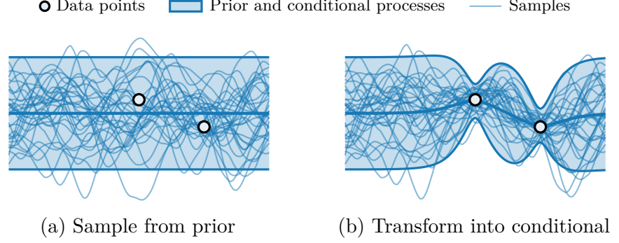
Figure 2.4. Illustration of pathwise conditioning of a Gaussian process. Here, we first sample a set of random functions from the prior, along with random noise variables at each of the data locations, then transform these into a samples from the posterior distribution. This view of conditioning is termed pathwise , since it is defined directly at the level of random functions.
