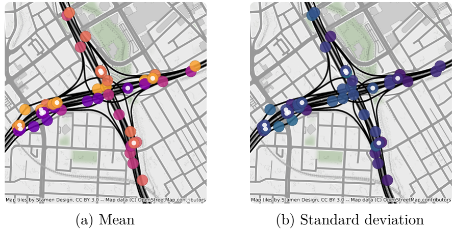
Figure 3.10. View of a zoomed-in portion of the posterior means and standard deviations of the probabilistic graph interpolation task on the road network. Note the small-scale variation present within the error bars.
