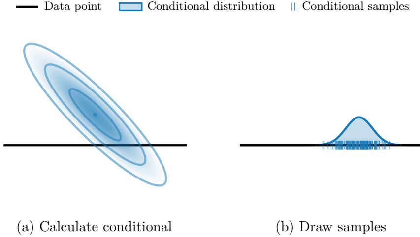
Figure 2.1. Illustration of distributional conditioning of a bivariate Gaussian. Here, we form the joint distribution, calculate the conditional distribution, and then draw samples from it. Note that all steps except the very last one are distributional in nature and do not involve the use of random variables, which only appear at the very end of the process.
