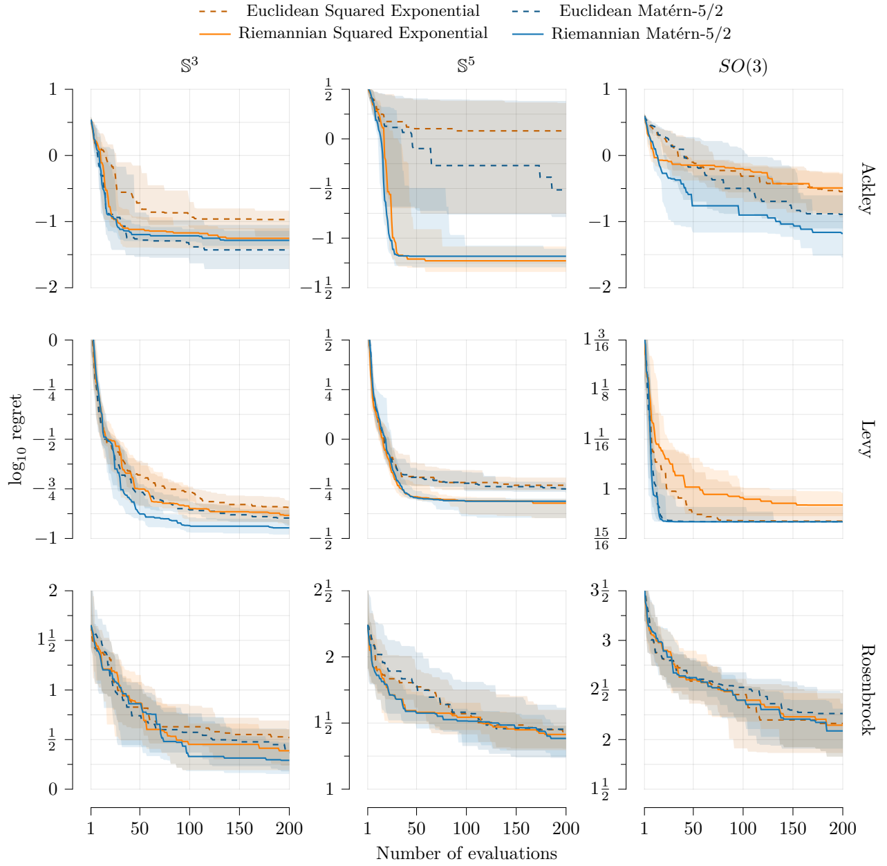
Figure 3.16. Geometry-aware Bayesian optimization benchmark results.
