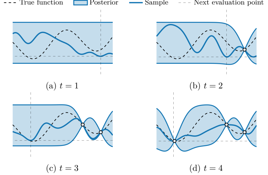
Figure 1.5. Bayesian optimization using Thompson sampling. Here, we sample a random function from the posterior distribution over possible functions, and choose the next evaluation point to be the minima of the sampled random function. As additional data is obtained, the posterior distribution concentrates around the true function. Unlike the upper confidence bound acquisition function considered previously, Thompson sampling makes use of a full probability distribution, rather than just a set of error bars.
