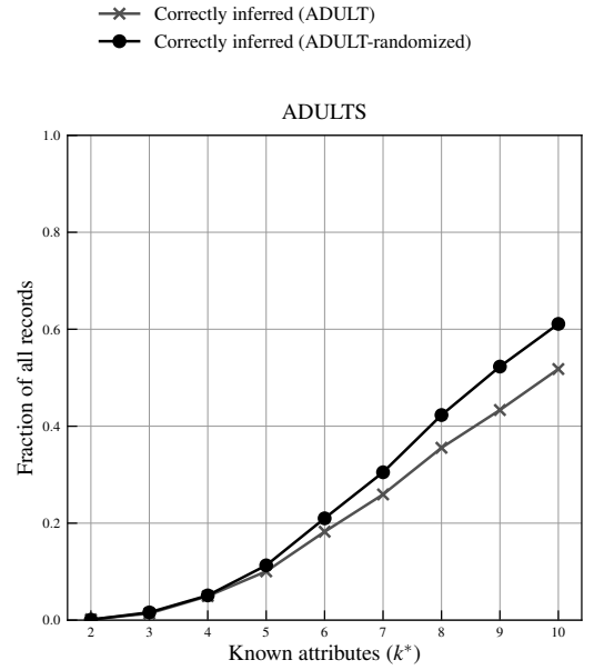
Figure 8: Results of the differential attack for the ADULT and the ADULT-randomized datasets.
