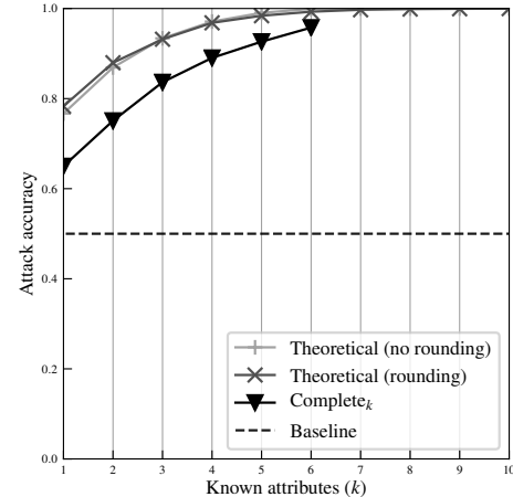
Figure 2: Accuracy of the differential attack when the uniqueness assumption is always validated and with balanced truth values. The baseline accuracy is 0.5 and represents the expected success rate when randomly predicting the secret attribute using a uniform prior.
