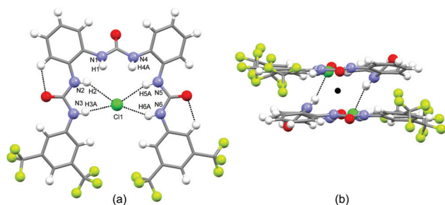
Fig. 2 Pseudo-cavity and main intermolecular interactions observed in structure L^5(Cl^-)(TBA^+) . (a) N-H\cdots Cl hydrogen bonds involving peripheral ureas and Cl^- . (b) N-H\cdots Cl hydrogen bonds involving central ureas and Cl^- and centro-symmetric dimer. The molecules are oriented to best show the intermolecular interactions. TBA^+ counter cations and positional disorder in the CF_3 groups are omitted for clarity. N-H\cdots O hydrogen bonds are indicated as black dashed lines, centre of inversion as black circle.
