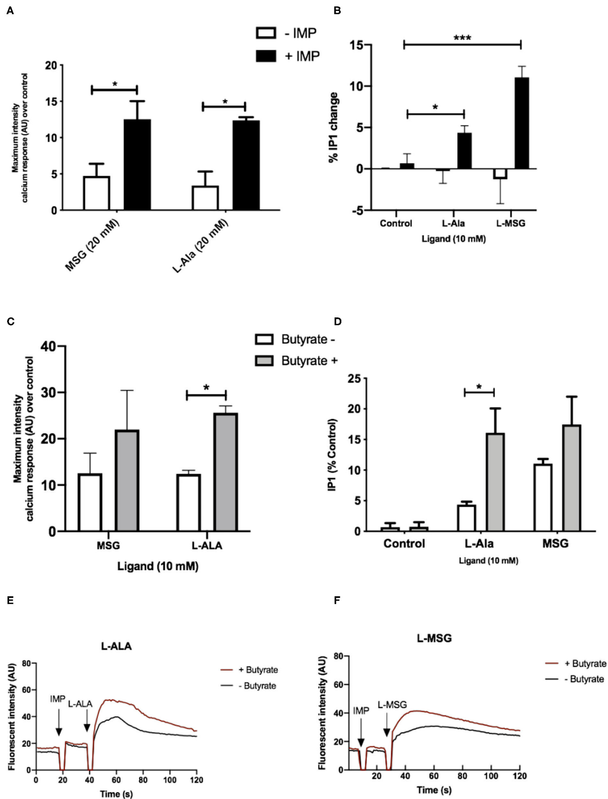
FIGURE 4 | Umami receptor signaling cascades are potentiated by butyrate pretreatment. (A) Intracellular \text{Ca}^{2+} levels measured in STC-1 cells, incubated with fluorescence \text{Ca}^{2+} indicator dye Fluo4-AM following addition of IMP (2 mM, black bars) or NaCl control (white bars; 2 mM) with L-Ala (20 mM) or L-MSG (20 mM).
