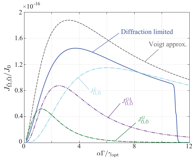
Figure 3. Numerical calculation (blue solid line) of J_{\Omega, \bar{\Omega}} and the corresponding Voigt based approximation (dashed grey line). A finely pixelated detector with N_p = 5000 pixels was assumed. The width of the response function of the dispersive element was taken as \gamma_{\text{disp}} = 8.4 nm and the relay lens assumed to have a numerical aperture of \text{NA} = 0.01 such that the spectrometer is diffraction limited. See Table 1 for other simulation parameters. Individual contributions to the Voigt approximation are shown by the dot-dashed light blue, green and purple lines corresponding to Eqs (37) (see also text), (51) and (55) respectively.
