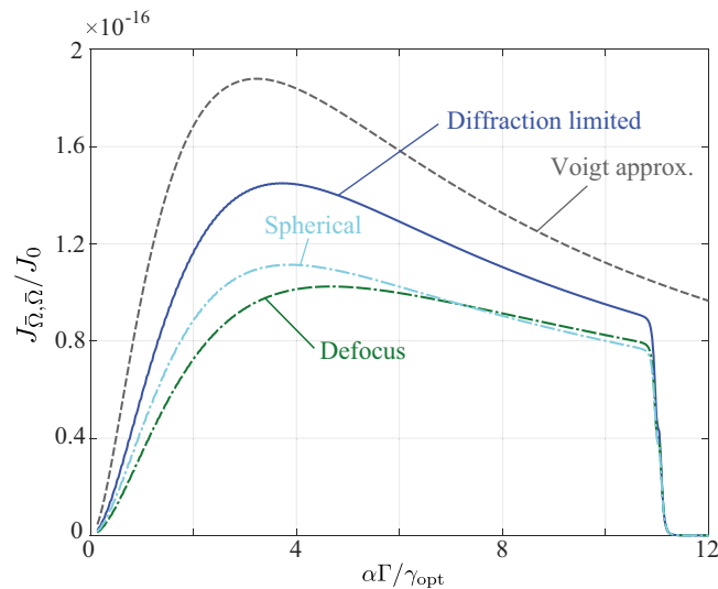
Figure 4. Numerical results (blue solid curve) for the diffraction limited case (as per. Fig. 3), with the addition of one wave of defocus (green dash-dotted curve) and spherical aberration (light blue dash-dotted curve). The Voigt based approximation is also shown by the grey dashed curve.
