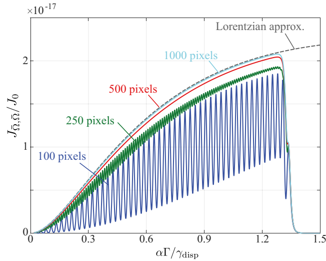
Figure 6. Calculated Fisher information in the coarse pixelation limit. Peak widths of \gamma_{\text{disp}} = 84 \mu\text{m} and \gamma_{\text{opt}} = 8.4 \mu\text{m} were assumed, whilst the number of pixels on a finite size detector was varied. Other simulation parameters are given in Table 1.
