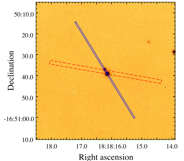
Figure 3. GMOS g' -band acquisition image of the central stars of IRAS 18153–1651, separated from each other by \approx 2.3 arcsec or \approx 0.02 pc in projection. The brightest of the stars is star 1. The relative positions of the GMOS and TWIN slits are shown by a solid (blue) and a dashed (red) rectangle, respectively. The widths of the rectangles of 0.75 and 2.1 arcsec correspond to the widths of the slits.
