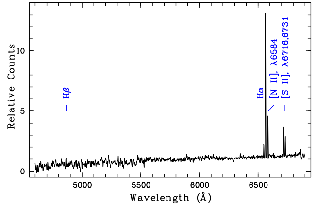
Figure 6. 1D spectrum of the optical arc obtained with the TWIN spectrograph.
