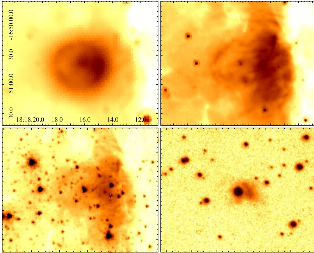
Figure 1. From left-hand to right-hand, and from top to bottom: Spitzer MIPS 24 \mu\text{m} and IRAC 8 and 3.6 \mu\text{m} , and SHS \text{H}\alpha + [\text{N II}] images of IRAS 18153–1651 and its central stars (the scale and orientation of the images are the same). The coordinates are in units of RA (J2000) and Dec. (J2000) on the horizontal and vertical scales, respectively. At a distance of 2 kpc, 1 arcmin corresponds to \approx 0.57 pc.
