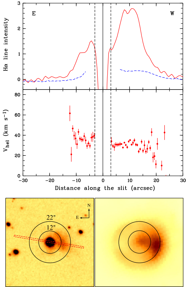
Figure 7. Upper panel: H\alpha line and continuum emission intensities along the TWIN slit ( PA = 80^\circ ), shown, respectively, with a solid (red) and dashed (blue) lines. Middle panel: H\alpha heliocentric radial velocity distribution along the slit. The E-W direction of the slit is shown. The solid vertical line corresponds to the position of star 1, while the dashed vertical lines (at \pm 3 arcsec from the solid one) mark the area where the radial velocity was not measured because of the effect of stars 1 and 2. Bottom panel: SHS H\alpha + [N II] (left) and MIPS 24 \mu m (right) images of IRAS 18153–1651 with the position of the TWIN slit shown by a red dashed rectangle. Concentric circles of radii 12 and 22 arcsec are overlaid on the images to make their comparison with the upper panels more convenient.
