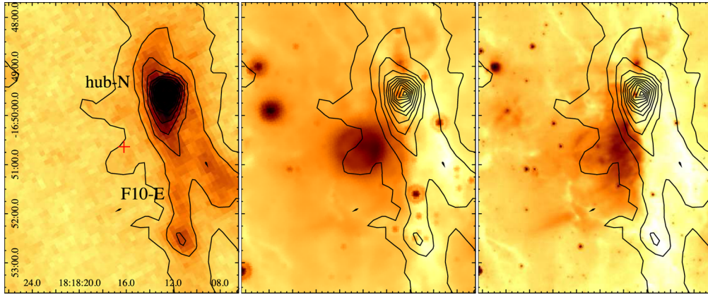
Figure 2. Left-hand panel: ATLASGAL 870 \mu\text{m} image of the region around IRAS 18153–1651, showing filamentary structures and a density enhancement (hub–N) at \approx 1.5 arcmin to the north–west from the position of stars 1 and 2 (indicated by a red cross). Middle and right-hand panels: Spitzer MIPS 24 \mu\text{m} and IRAC 8 \mu\text{m} images of the same region with the 870 \mu\text{m} image overlaid in black contours. The coordinates are in units of RA (J2000) and Dec. (J2000) on the horizontal and vertical scales, respectively. At a distance of 2 kpc, 1 arcmin corresponds to \approx 0.57 pc. See text for details.
