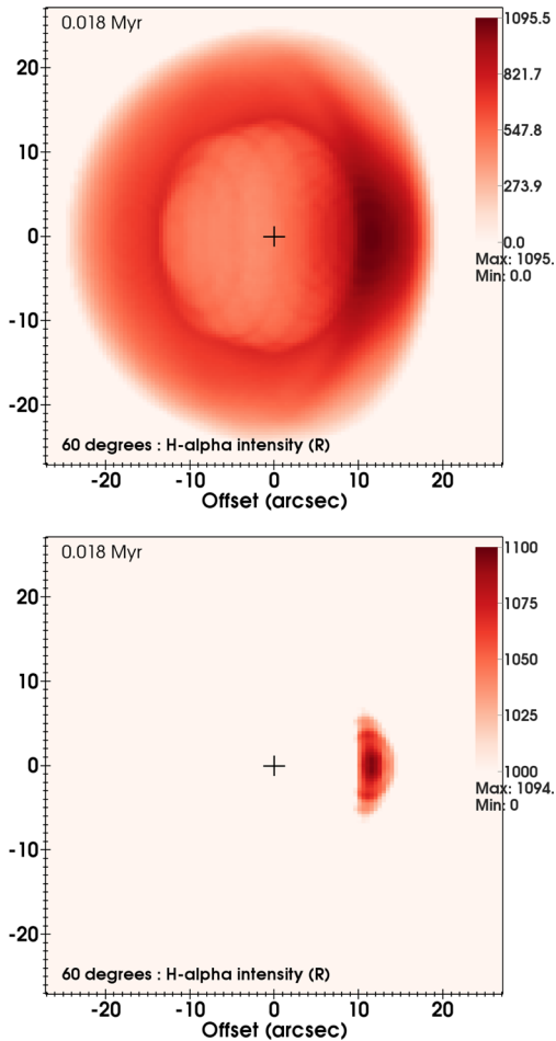
Figure 10. H\alpha emission maps calculated with VISIT , for an angle of 60^\circ to the symmetry axis of the simulation. The upper panel shows the predicted H\alpha surface brightness in R on a linear scale (although the absolute brightness should be treated with caution). The bottom panel shows only the brightest 10 per cent of the predicted emission to mimic the case where the brightest emission is just above the noise level. A cross at the origin shows the location of the B1 star.
