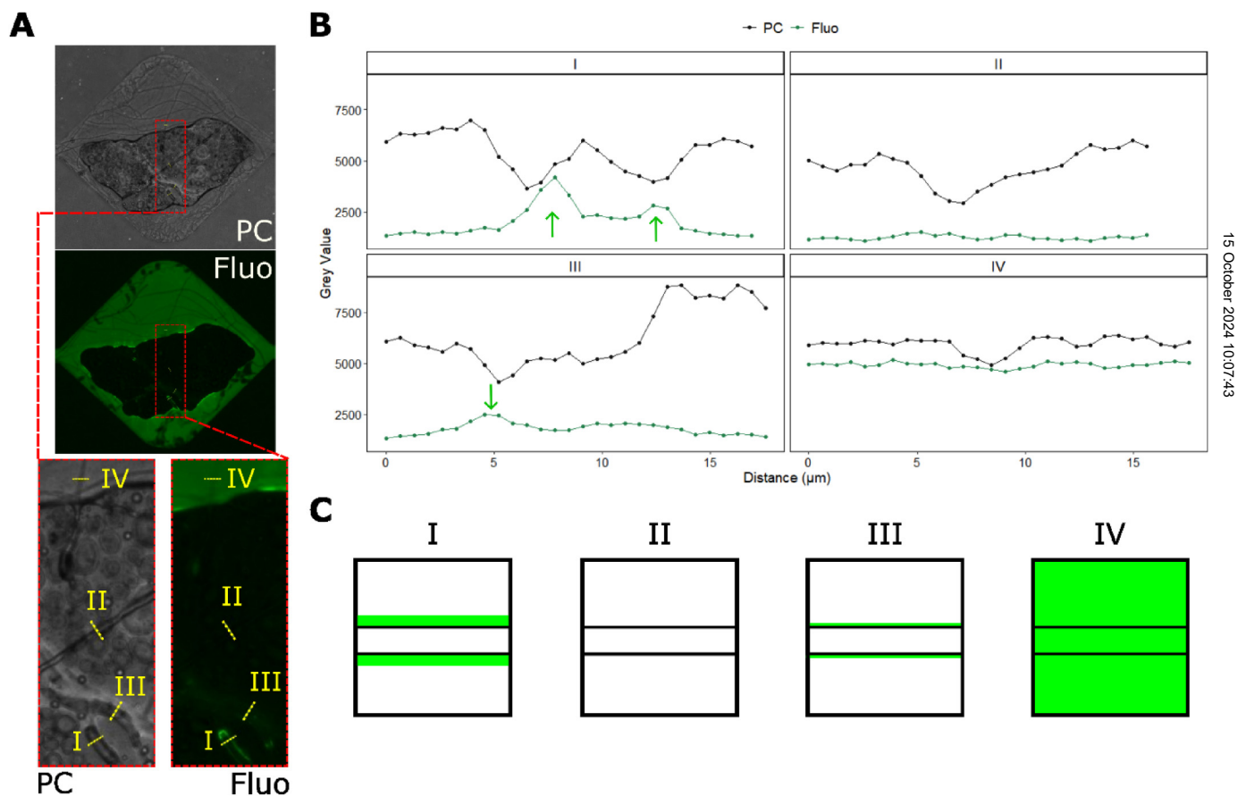
FIG. 3. (a) Phase contrast (PC) and fluorescence (fluo) microscopy image of P. ultimum and fluorescein at day 7 post-inoculation. Dashed red boxes and lines indicate the close up images of the corresponding larger image. In ImageJ, the “line” tool was used to draw the profile lines across hyphae (as indicated by the yellow dashed lines) and subsequently measure the gray value every 0.65 \mu\text{m} . (b) Graph shows the gray value of each hypha, as labeled in (a) and represented in (c), over the distance of the measurement line. Green arrows highlight the peaks in the gray value of the fluorescence images that correspond to where the liquid film is present. (c) Schematic illustrating the different hyphae labeled in (a) and measured in (b). The hyphae were classified as (I) surrounded by an easily visible, thicker liquid film; (II) not surrounded by a visible liquid film; (III) surrounded by a poorly visible, thinner liquid film; or (IV) saturated in liquid.
