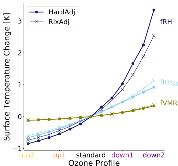
FIG. 5. Surface temperature changes corresponding to artificially shifted ozone profiles, with negative surface temperature changes on the left corresponding to an upward shift (yellow in Figure 4) and positive temperature changes on the right to a downward shift (purple in Figure 4). Dots and crosses correspond to experiments with the hard convective adjustment (HardAdj) and the relaxed adjustment (RlxAdj) respectively. The different colours of the lines and markers are for the different treatment of water vapour. The standard treatment, with fixed relative humidity in the troposphere and stratospheric humidity set by the cold point, is indicated by fRH. Runs with fixed relative humidity in the troposphere but a constant specified stratospheric water vapour mixing ratio are labeled as fRH 55 . Runs with a fixed water vapour volume mixing ratio at each pressure level throughout the column are labeled as fVMR.
