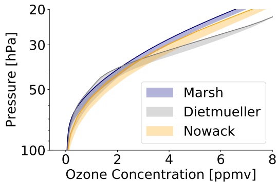
FIG. 10. Tropical mean lower stratospheric ozone profiles from the coupled chemistry climate models of Marsh et al. (2016), Dietmüller et al. (2014) and Nowack et al. (2014). The solid lines indicate the profiles in the 4 \times \text{CO}_2 scenarios, and the shading shows the change from the 1 \times \text{CO}_2 runs.
