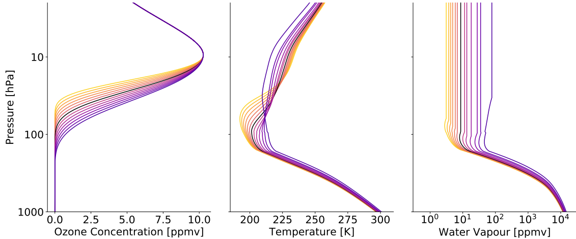
FIG. 4. Artificial changes to the ozone concentration profile (left) and the corresponding changes to the temperature and water vapour profiles for the hard convective adjustment case. The black lines indicate the standard profiles, and the yellow correspond to an upward shift in the ozone profile, as might be expected under global warming.
