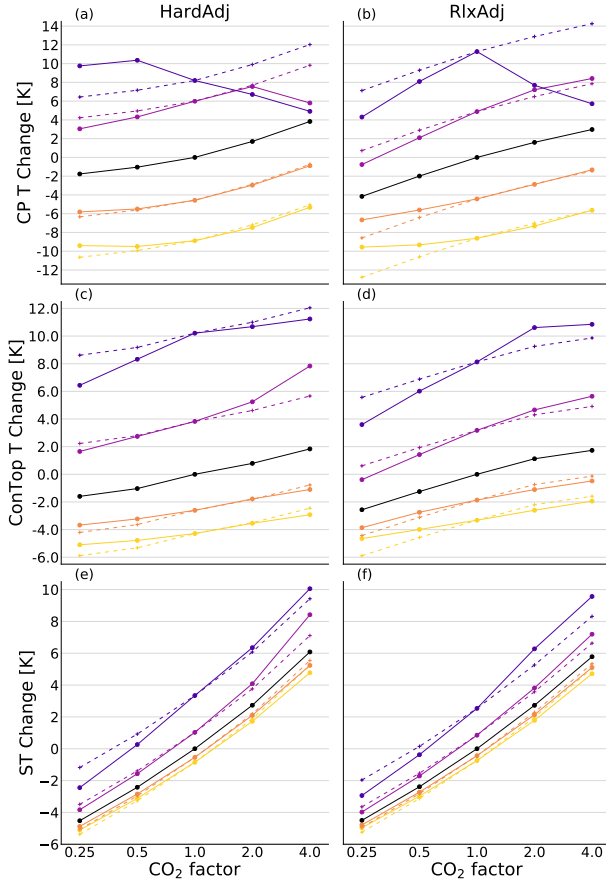
FIG. 7. Cold point (top row), convective top (middle row) and surface (bottom row) temperature changes with increasing \text{CO}_2 and different ozone profiles. The ozone profile used is indicated by the color, with black representing the standard profile, pink and purple representing downward shifted profiles (those indicated as down1 and down2 in Figure 5) and orange and yellow representing upward shifted profiles (up1 and up2 respectively). Results for the set-up with the hard convective adjustment are shown on the left, and those with the relaxed convective adjustment on the right. Dashed lines and crosses show the predicted behaviour assuming additivity and solid lines and dots show the actual behaviour.
