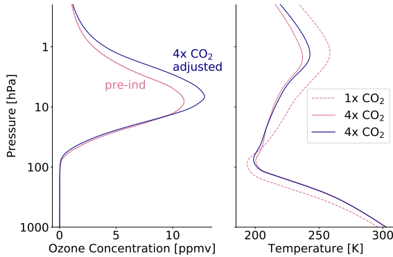
FIG. 9. Temperature profiles (right) from our 1D RCE when using the ozone profiles (left) from Marsh et al. (2016). The dashed pink temperature profile is from that found for the run with 1 \times \text{CO}_2 and the pre-industrial ozone profile (pink, left panel). The solid pink and blue temperature profiles are from runs with 4 \times \text{CO}_2 and the ozone profiles of corresponding colours.
