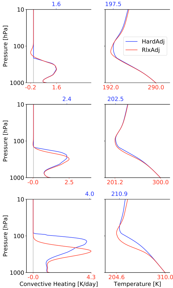
FIG. 2. Convective heating rate and temperature profiles for the hard (blue) and relaxed (red) convective adjustments with surface temperatures fixed at 290 K (top row), 300 K (middle row) and 310 K (bottom row). Surface and cold point temperatures are indicated, as are minimum and maximum convective heating rates.
