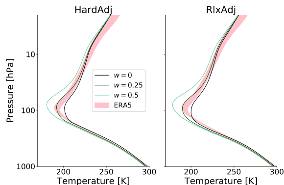
FIG. 6. Temperature profiles for runs with different stratospheric upwelling velocities. The standard set-up with no upwelling is shown in black and runs with upwelling velocities of 0.25 and 0.5 \text{mm s}^{-1} are shown in dark and light green respectively. Pink shading shows ERA5 reanalysis data within one standard deviation of the mean tropical temperature profile.
