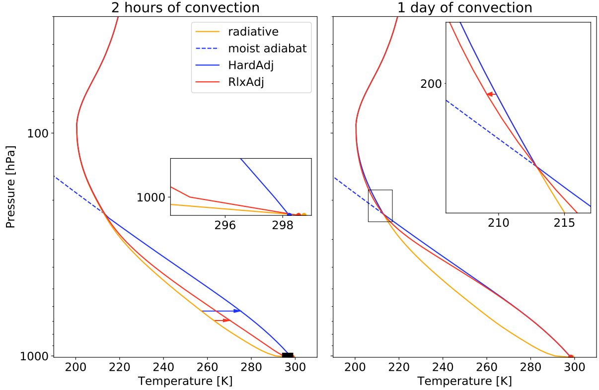
FIG. 1. A comparison of the hard adjustment (HardAdj, blue) and the relaxed convective adjustment (RlxAdj, red), with the radiative profile shown in orange. The radiative profile results from turning off convection for 20 model days: it is not radiative equilibrium, nor is it the radiative profile after a single model iteration, which would barely differ from radiative-convective equilibrium. The left panel shows the convectively adjusted profiles after 2 model hours of convection and the right panel after 1 day of convection. The zoom box of the left panel shows the region close to the surface (black rectangle on the main plot), with surface temperatures indicated by dots. The zoom box of the right panel shows the region around the top of convection, above which HardAdj is equal to the radiative profile, but RlxAdj is between the radiative profile and the moist adiabat. The horizontal blue and red arrows show \Delta T_{\text{hard}}(p) and \Delta T(p) = \Delta T_{\text{hard}}(p) \times R(p) respectively.
