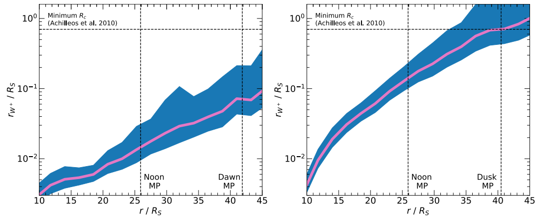
Figure 4. The water group ion gyroradius r_{w+} is shown as a function of radial distance for the dawn (left) and dusk (right) local time sectors. The horizontal dashed lines show the minimum expected radius of curvature. The vertical dashed lines show the average nose standoff distance for our five cushion examples and the mapped terminators. The pink line shows r_{w+} calculated using the average magnetic field strength. The blue region shows r_{w+} calculated using the standard deviations of the mean magnetic field. These results show that r_{w+} approaches R_C at dusk at distances between noon and the terminator, but at dawn it far less likely to.
