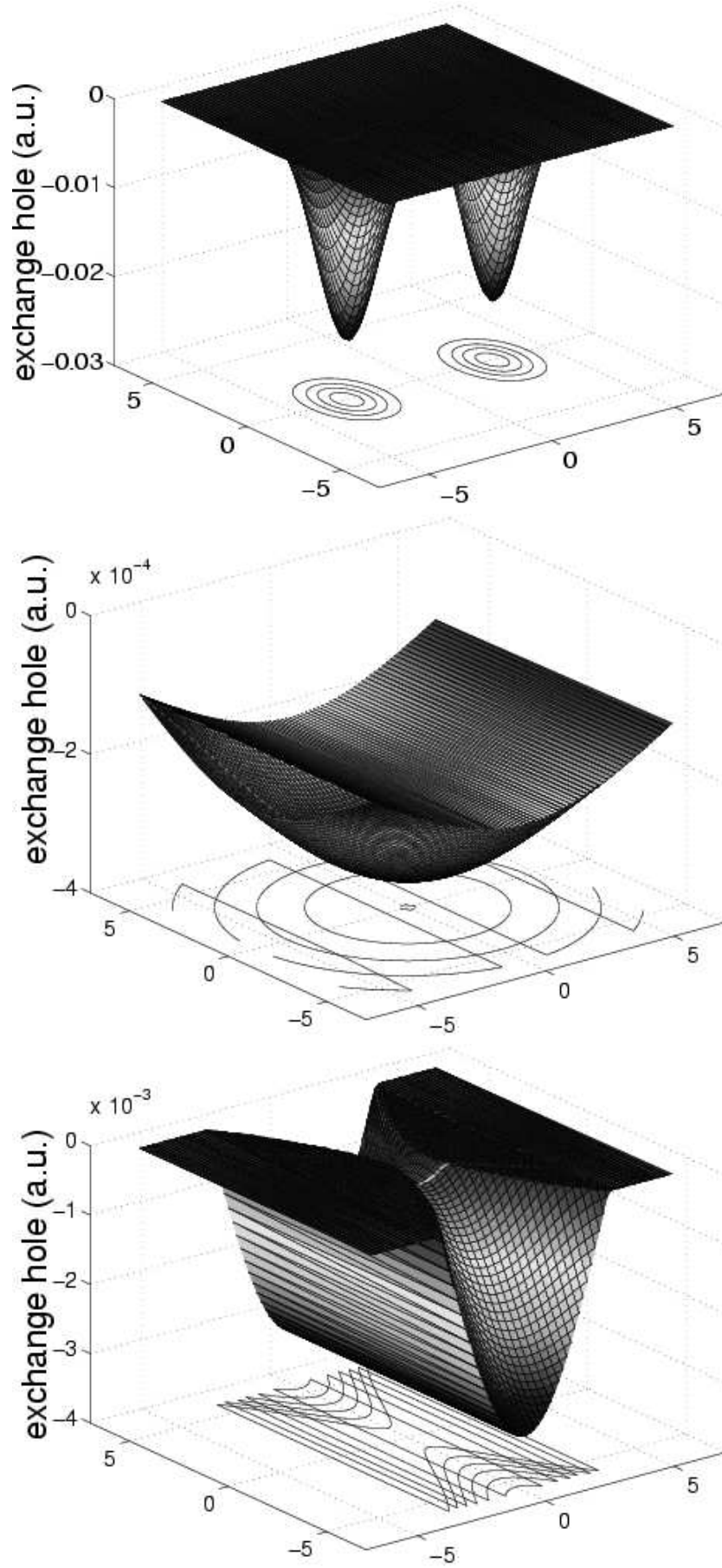
FIG. 5: The exact, LDA and truncated GEA exchange holes, n_x(\mathbf{r}, \mathbf{r} + \mathbf{R}) , for the strongly inhomogeneous q = 1.1080k_F^0 system plotted for \mathbf{r} at a density minimum and \mathbf{R} ranging in a plane parallel to \mathbf{q} . Distances are in atomic units.
