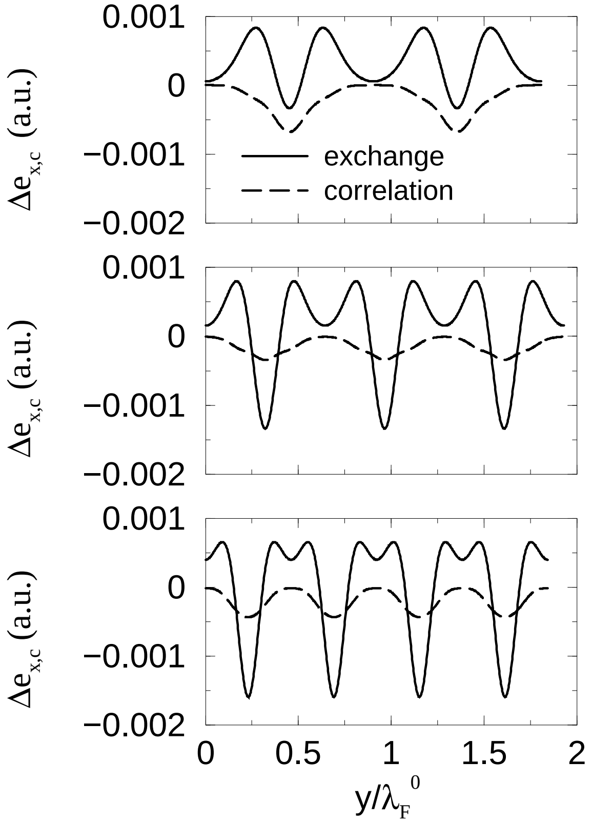
FIG. 7: The differences e_x^{LDA} - e_x^{VMC} (solid lines) and e_c^{LDA} - e_c^{VMC} (dashed lines) are shown along a direction parallel to \mathbf{q} for (from top to bottom) the q = 1.1080k_F^0 , q = 1.556k_F^0 , and q = 2.172k_F^0 systems.
