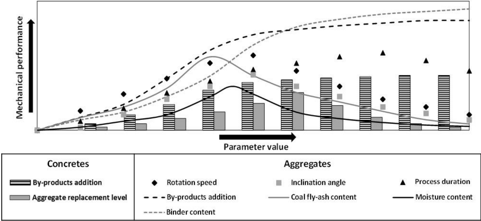
Fig. 2. Exemplifying graphical representation of qualitative variation trends for aggregate (dots and lines) and concrete (histograms) mechanical performance at different values of the operating parameters. Parameter values increase from left to right side and mechanical performance improvement from down to up side.
