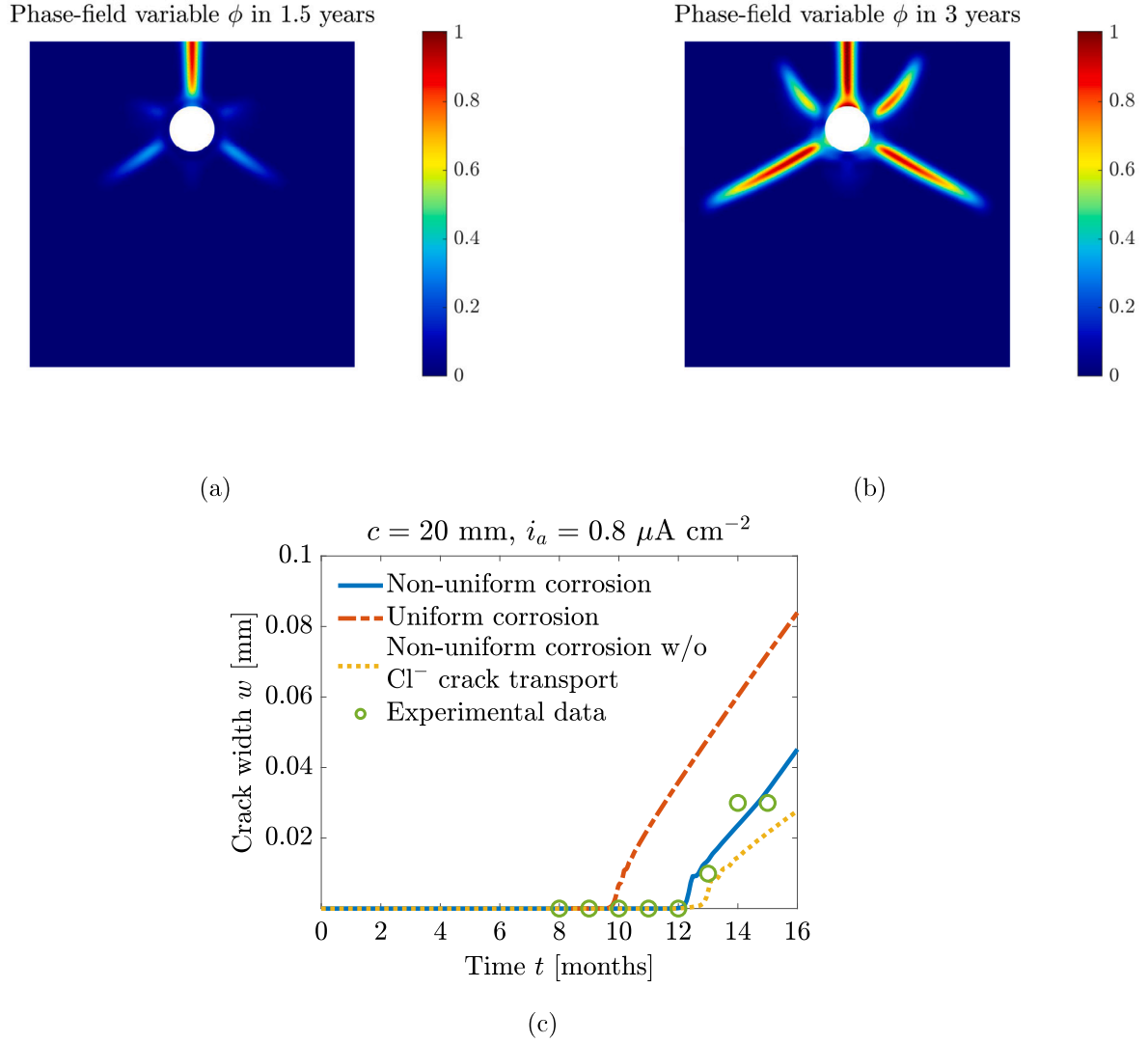
Fig. 4. Predicted growth and nucleation of cracks for the work of Chen et al. [16] characterised by the contours of the phase-field variable \phi in (a) 1.5 and (b) 3 years. The evolution of surface crack width predicted by the proposed non-uniform model is compared with experimental measurements of Chen et al. [16] (c). The comparison with alternative predictions of the uniform corrosion model and non-uniform corrosion model neglecting the transport of chloride through cracks stressing the importance of corrosion non-uniformity and crack-facilitated chloride transport is also provided in (c).
