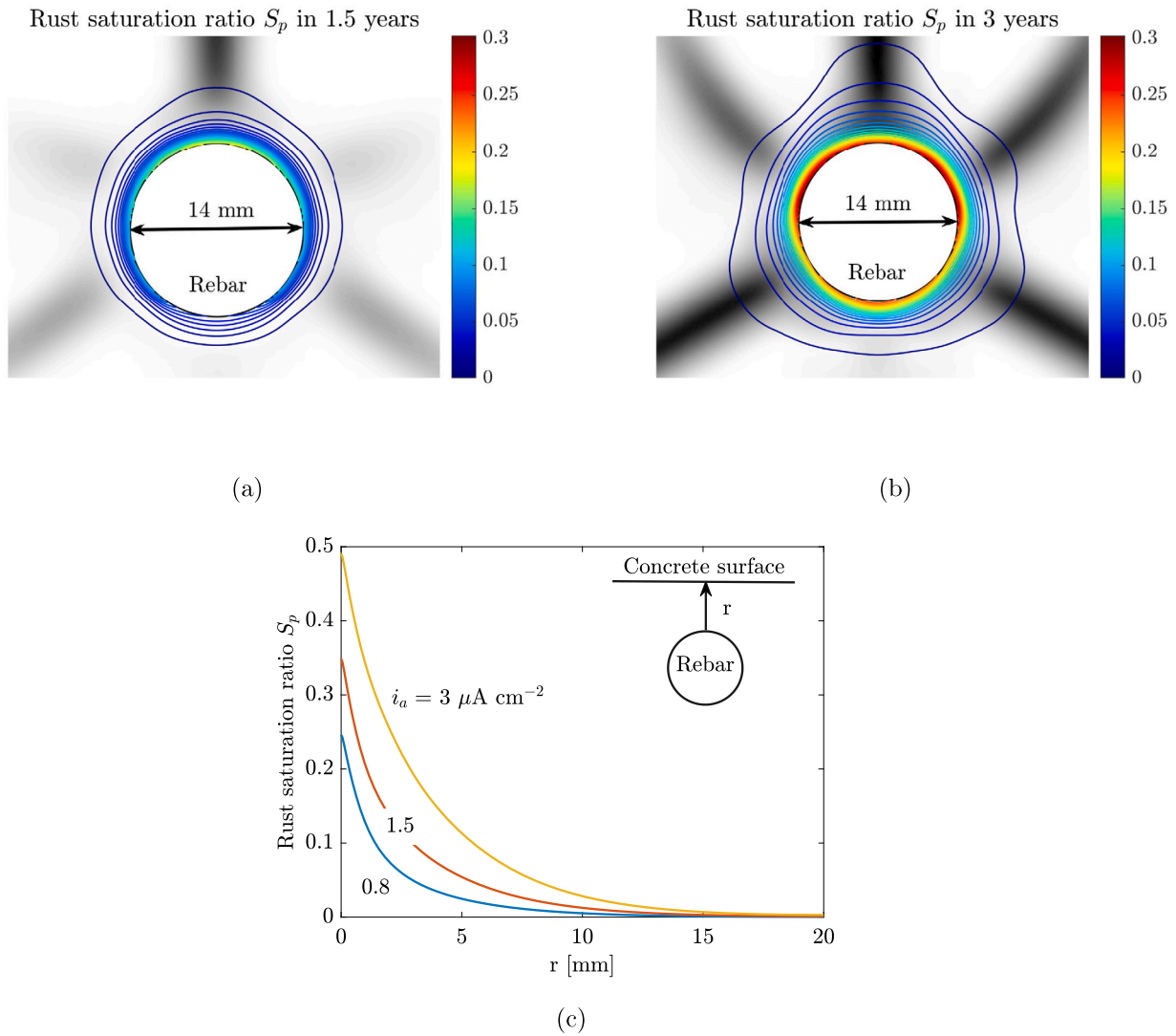
Fig. 6. Contours of the precipitate saturation ratio S_p in the vicinity of rebar for the test of Chen et al. [16] in (a) 1.5 years and (b) 3 years reveal that even in three years time only 30% of the concrete pore space surrounding the rebar is filled with precipitates, suggesting that the studied driving mechanism of corrosion-induced fracture, i.e., the accumulation of rust under constrained conditions in concrete pore space, could dominate for years under the low corrosion current densities of natural chloride-induced corrosion. The phase-field variable \phi is shown in the back in a grey scale bar (0 – white, 1 – black). The comparison of the evolution of S_p in a radial direction from the rebar ( r, \theta = 0^\circ ) for corrosion current densities 0.8, 1.5 and 3 \mu\text{A cm}^{-2} shows that even for values of corrosion current density that are 3.5 times higher than those considered in the simulation of the tests of Chen et al. [16], only less than half of the pore space is filled with precipitates in this radial section.
