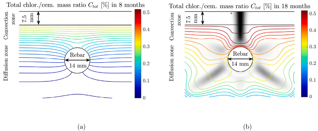
Fig. 5. The contours of total chloride content C_{tot} for the test of Chen et al. [16] in 8 months (a) and 18 months (b) revealing the profound impact of cracks on chloride transport through concrete. The phase-field variable \phi is shown in the back in a grey scale bar (0 – white, 1 – black).
