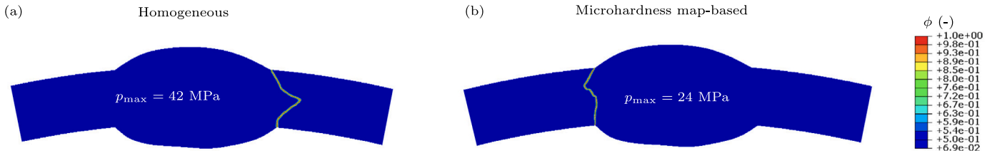
Fig. 15. Investigating the role of accounting for the microstructural heterogeneity of seam welds. Cracking (phase field) contours for: (a) the case where material properties are considered to be homogeneous in the weld and base metal regions, and (b) the case where material properties are varied according to the microstructural hardness map (see Figs. 4 and 13). Failure takes place due to cracking at critical pressures of p_{\max} = 42 MPa and p_{\max} = 24 MPa, respectively.
