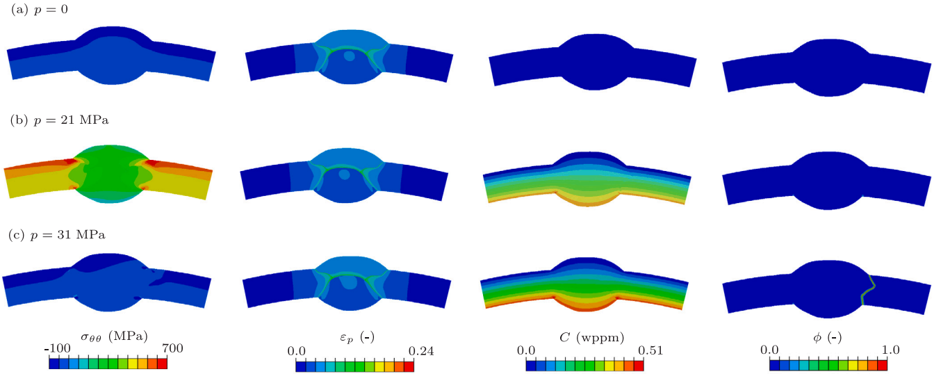
Fig. 7. Predictions of circumferential stress ( \sigma_{\theta\theta} ), accumulated plastic strain ( \epsilon_p ), lattice hydrogen concentration ( C ), and phase field fracture ( \phi ) as a function of the pipeline pressure: (a) initial state ( p = 0 ), (b) p = 21 MPa, and (c) p = 31 MPa. Results obtained for the two-pass weld considering X80 pipeline steel as the base and weld materials.
