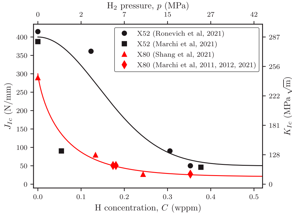
Fig. 3. Hydrogen-dependent critical fracture energy for API steels: X52 [64,65], X80 [66–69]. The fitted curves are obtained using Eq. (17) with fitting parameters listed in Table 2. For convenience, the corresponding critical stress intensity factor K_{Ic} is added on the right and it is related to J_{Ic} , as K_{Ic} = \sqrt{E'J_{Ic}} with E' = E/(1 - \nu^2) for plane strain conditions. Also the corresponding hydrogen pressure p is added on top; lattice hydrogen concentration C and hydrogen pressure p are related via Sievert's law C = S\sqrt{p} , with the solubility of steel taken to be S = 0.077 wppm MPa -0.5 [70].
