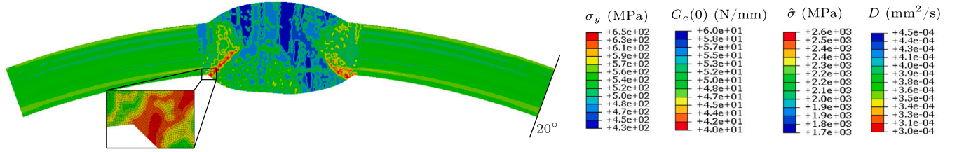
Fig. 13. Spatial distribution of relevant material properties (yield stress, toughness, strength and diffusivity) as inferred from the microhardness map of the three-pass weld (see Fig. 4). The results shown correspond to the X52 pipeline steel case.
