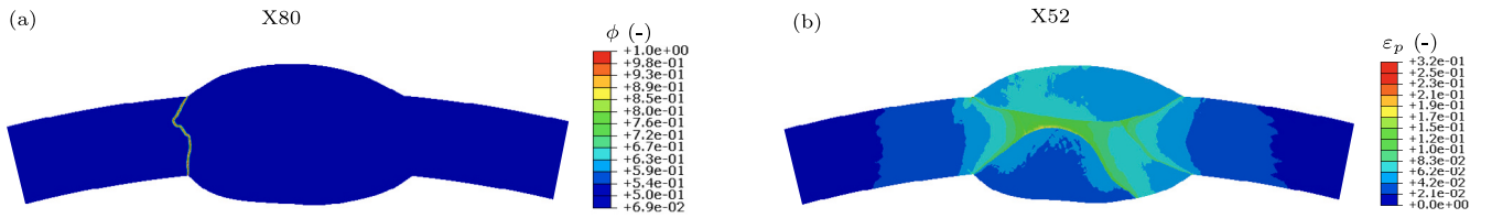
Fig. 14. Computational predictions of weld structural integrity in hydrogen transport pipelines: (a) brittle fracture in an X80 pipeline at a critical pressure of p_{\max} = 24 MPa, (b) failure by global plastic yielding in an X52 pipeline.
