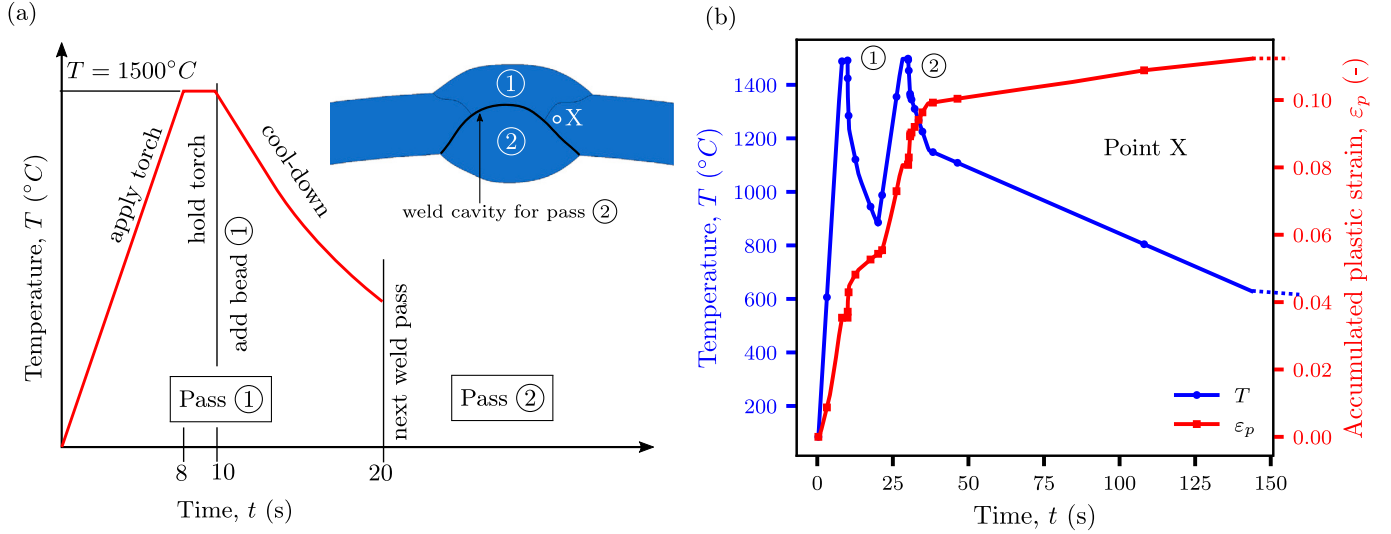
Fig. 5. Two-pass weld welding process modelling: (a) schematic representation of the temperature boundary conditions for a two-pass weld; and (b) thermal loading history and corresponding accumulated plastic strain at point 'X' near the weld. Only the first 150 s are shown but the simulation is continued until reaching room temperature (20 °C).
