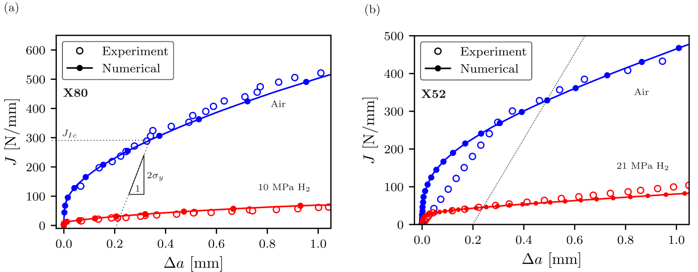
Fig. A.2. Predicting the crack growth resistance behaviour of (a) X80 pipeline steel [66], and (b) X52 pipeline steel [63], in both air and hydrogen environments.
