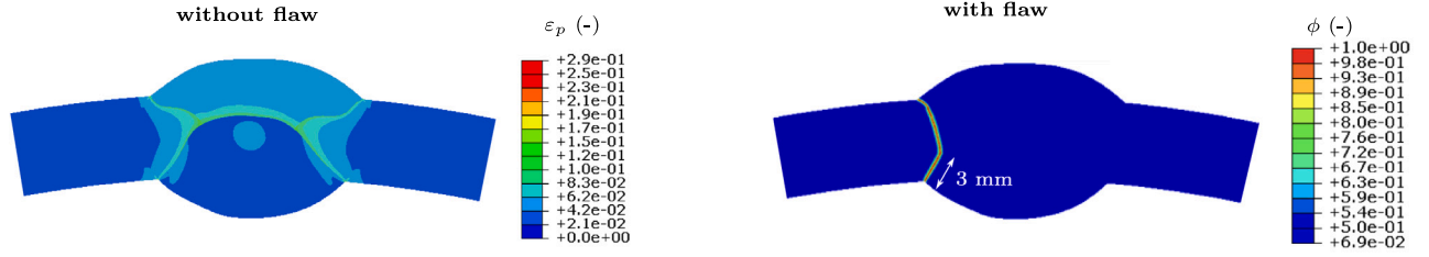
Fig. 12. Investigating the role of an external pre-existing flaw that is located near the inner surface and aligned with the HAZ. Results obtained for the two-pass weld considering X52 pipeline steel as the base and weld materials. The finite element analysis reveals: a global yielding type of failure at p_{\max} \approx 29 MPa in the absence of flaws (a), yet a brittle fracture event at a pressure of p_{\max} = 19 MPa in the presence of a 3 mm flaw along the HAZ (b).
