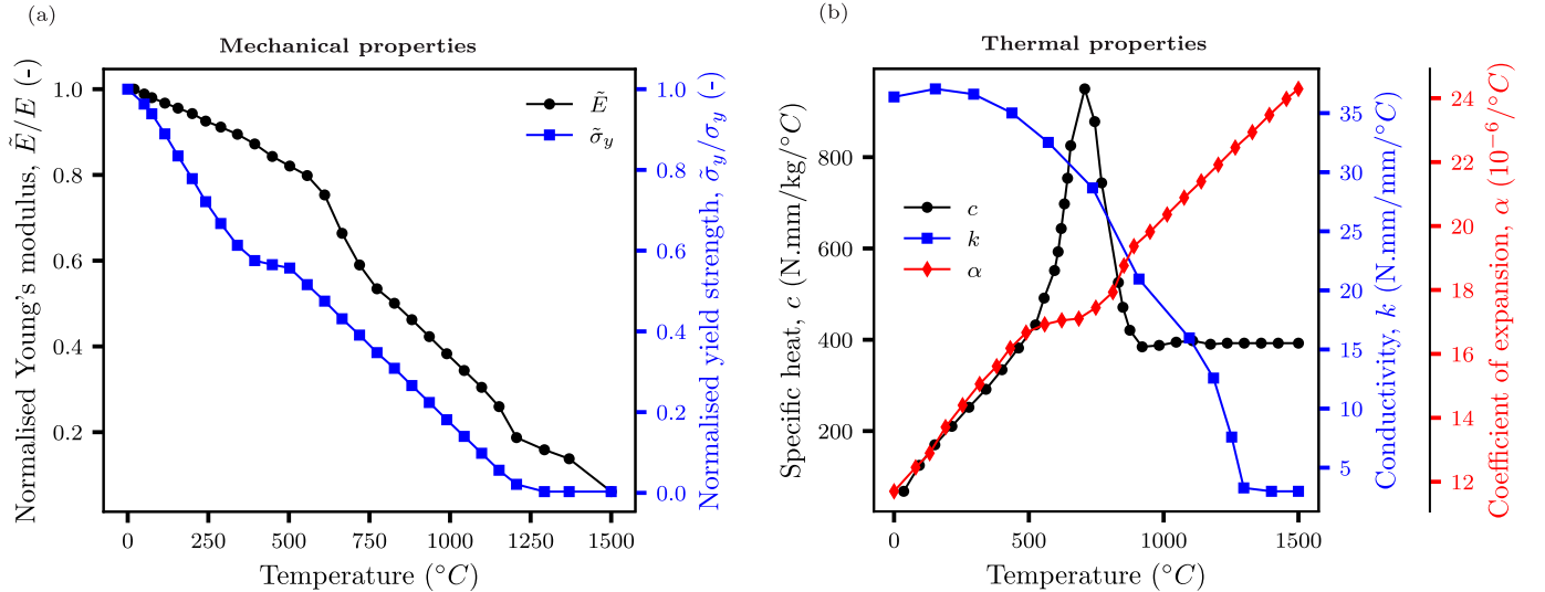
Fig. 2. Temperature-dependence of the material properties of carbon steel SA-516 Grade 70, as per ASME, Section 2, Part D [48]. The normalised mechanical properties are presented in (a), where E and \sigma_y denote Young's modulus and yield strength at room temperature, respectively, and \square represents the corresponding temperature-dependent parameter. The temperature dependence of the thermal properties (specific heat c , conductivity k , coefficient of thermal expansion \alpha ) is given in (b).
