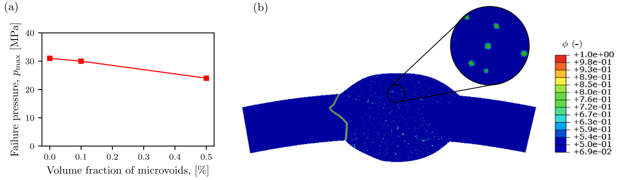
Fig. 9. Investigating the role of porosity on the failure of hydrogen transport pipelines: (a) sensitivity of the critical failure pressure to the void volume fraction, and (b) cracking pattern (phase field contours) observed for a volume fraction of 0.5%, which corresponds to a critical pressure of p_{max} = 24 MPa. Results obtained for the two-pass weld considering X80 pipeline steel as the base and weld materials.
