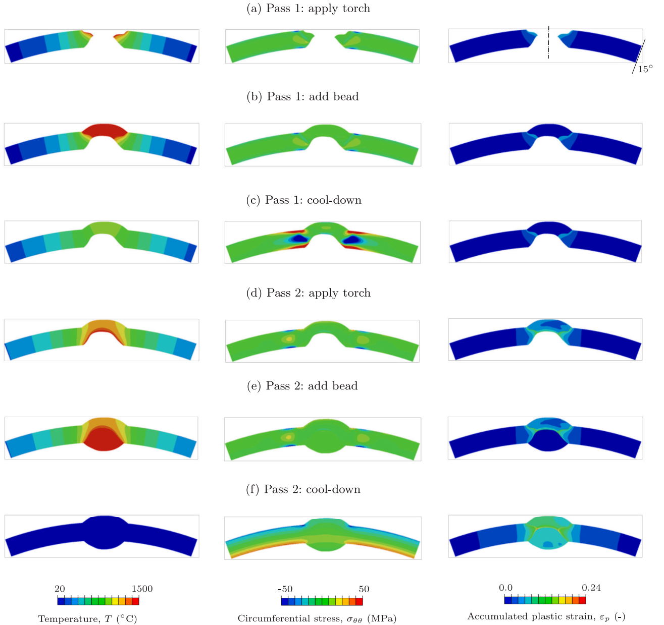
Fig. 6. Evolution of temperature, residual stress and plastic strain in the two-pass welding process. This set of representative results has been obtained for X52 pipeline steel.
