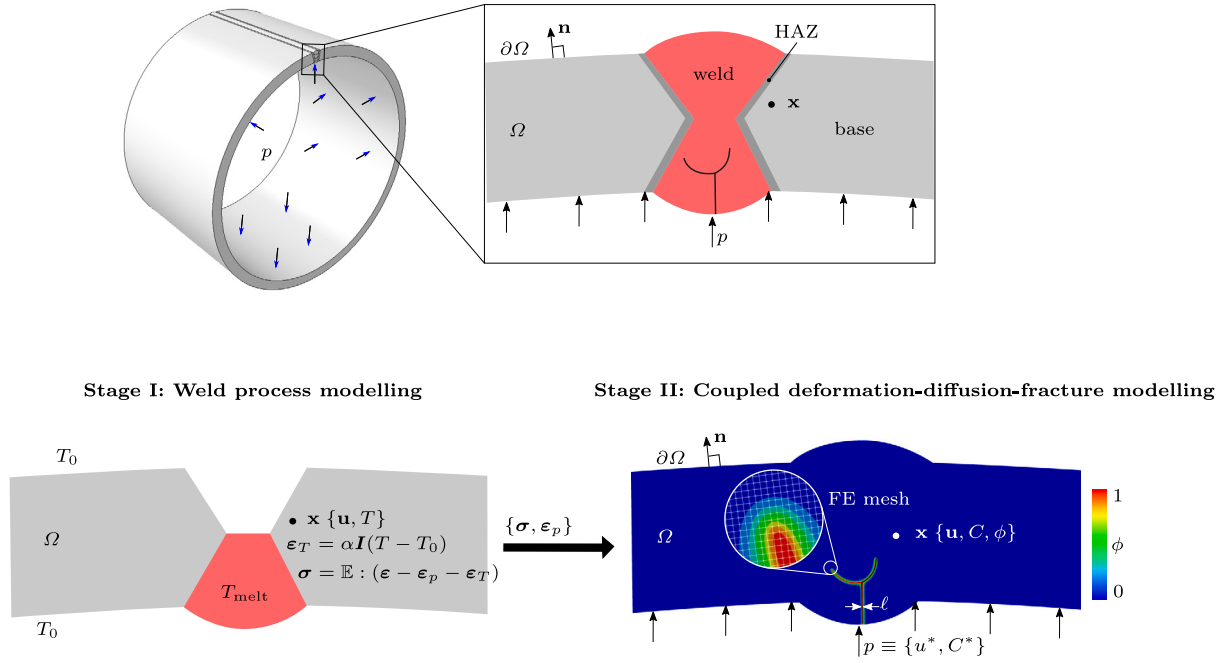
Fig. 1. Schematic representation of the finite element modelling framework, aimed at predicting hydrogen-assisted failures of welded joints in pipelines subjected to an internal hydrogen pressure p . The first stage of the modelling framework handles the simulation of the welding process, as illustrated here with one weld bead at initial melting temperature T_{\text{melt}} . The second stage uses a coupled, multi-physics phase field formulation to represent the nucleation and growth of cracks, as assisted by hydrogen.
