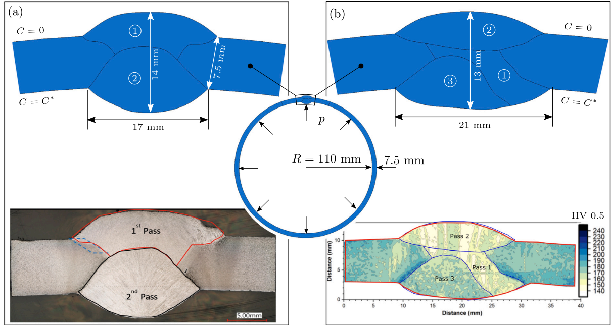
Fig. 4. Schematic representation of the boundary value problem considered, a pipeline containing a longitudinal weld. Two weld configurations were employed based on images of ex-service welds from natural gas pipelines: (a) a two-pass weld of dimensions 17 \times 14 mm, and (b) a three-pass weld of dimensions 21 \times 13 mm. The microstructural heterogeneity of the second weld was characterised using a Vickers Hardness (VH) mapping approach. The associated chemical boundary conditions, including the internal exposure to a hydrogen concentration C^* , are also displayed.
