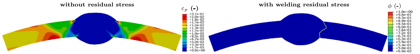
Fig. 8. Investigating the role of welding residual stresses on the failure of hydrogen transport pipelines: in the absence of residual stresses plastic failure occurs (left, \epsilon_p contours), while when residual stresses are accounted for cracking is observed (right, \phi contours). Results obtained for the two-pass weld considering X80 pipeline steel as the base and weld materials.
