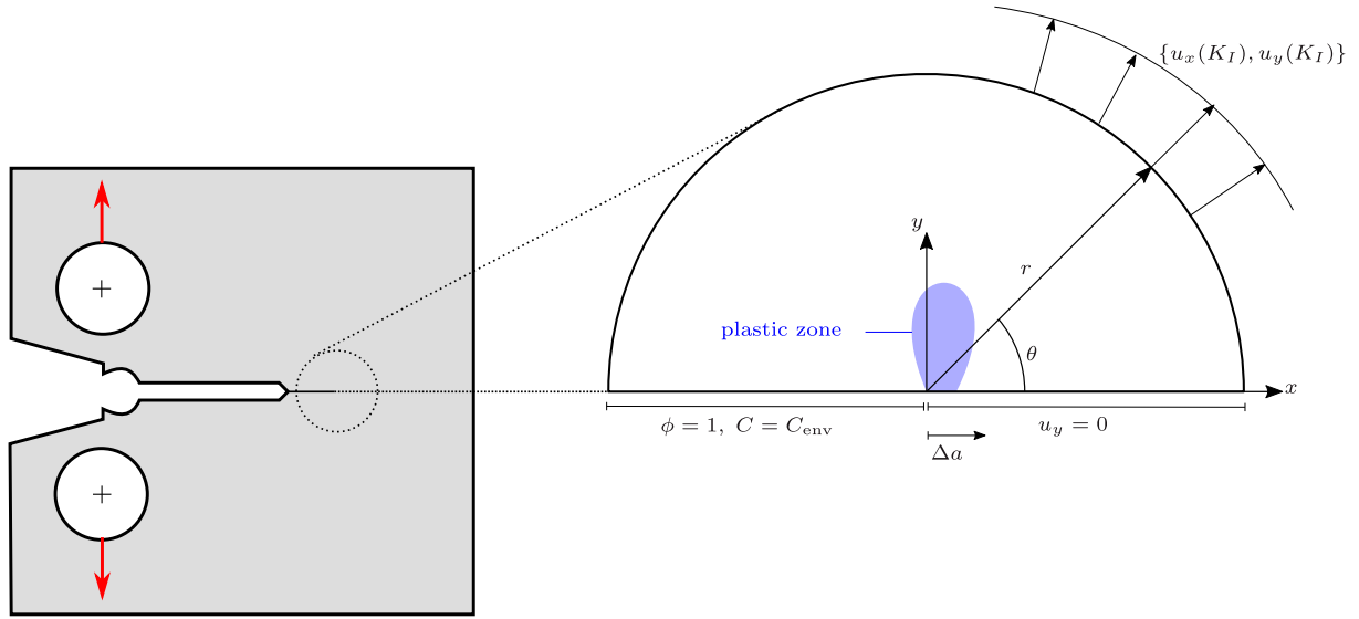
Fig. A.1. The boundary layer idealisation of a compact tension specimen under small-scale yield conditions. R-curves are obtained by applying a remote K(J) and measuring the crack extension \Delta a .
