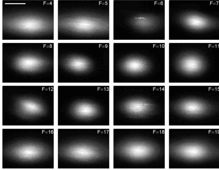
Figure 2.5: Mode profiles on chip ORC1. The writing fluence (in \text{J}/\text{cm}^2 ) is indicated on each image. The scale is indicated by the 5\text{ }\mu\text{m} long white line in the first image.
