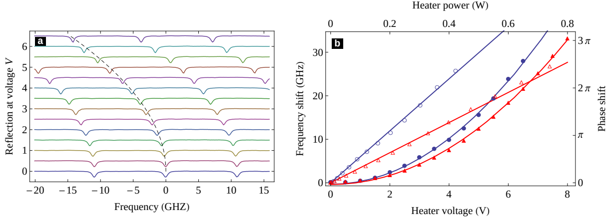
Figure 3.6: (a) Frequency shift of a waveguide cavity reflection spectrum as a function of heater voltage (indicated on the vertical axis.) (b) Frequency shift \Delta f and phase shift ( \Delta\phi = \pi\Delta f/FSR ) as a function of heater voltage V and power V^2/R . The red curves correspond to the spectra on the left (wire length 1.5 mm, resistance R = 110\ \Omega ). The blue curves are for a different heater (1.1 mm, 75\ \Omega ).
