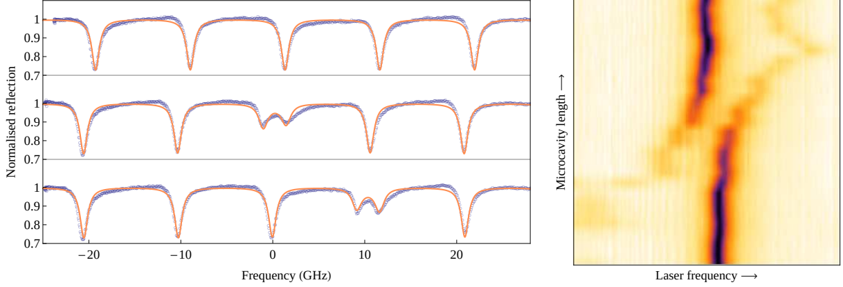
Figure 4.6: Observation of waveguide-microcavity coupling on ORC7. Top: the microcavity is far detuned and we only observe the waveguide spectrum. Middle and bottom: the microcavity is tuned to two different waveguide resonances. The solid lines are fits to Eq. (4.3), including waveguide and mode matching losses. Right: scanning the laser frequency and the microcavity length reveals that the observed splitting is a proper avoided crossing. The frequency and length axes span about 8 GHz and 50 nm respectively (the exact calibration is not available).
