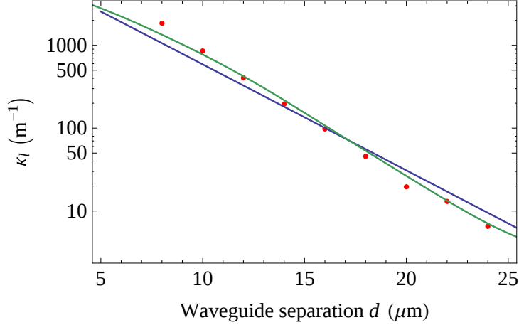
Figure 2.11: Coupling constant \kappa_l as a function of waveguide separation d , according to the three methods outlined in the text. Green curve: integral overlap method for a 5\ \mu\text{m} square waveguide, calculated with MPB. Red dots: direct MPB simulation (Eq. (2.12)), with the same parameters. Blue curve: Snyder’s analytical formulae Eq. (2.14) for a cylindrical fibre of diameter 5\ \mu\text{m} . The index contrast was \Delta n = 0.004 .
