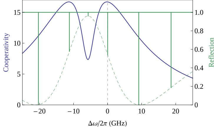
Figure 4.4: Cooperativity of a Rb atom in a microcavity coupled to a waveguide cavity ( R_w = 0.98, L_w = 23 \text{ mm}, R_{cw} = 0.98, L_c = 156 \mu\text{m}, R_c = 0.999 ). Both cavities have been tuned to bring a resonance (green lines, dashed envelope) and maximise the cooperativity at the atomic frequency at \Delta\omega = 0 .
