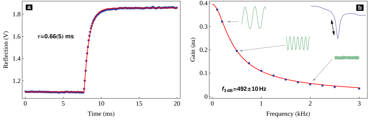
Figure 3.7: Measurement of a phase shifters' response time. (a): the laser sits on the side of a resonance fringe, and a small square modulation is applied to the heater. (b): the modulation is now sinusoidal, and the signal's modulation amplitude is recorded as a function of modulation frequency. It is then fitted with a simple first-order, low-pass filter gain function. The half-maximum cut-off frequency is 492(10) Hz.
