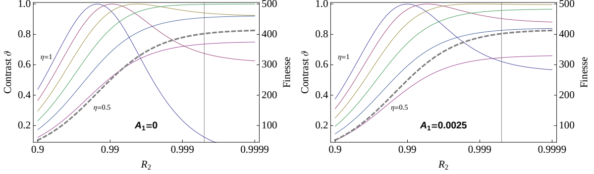
Figure 3.2: Contrast \vartheta of the reflection fringes of a Fabry-Pérot cavity as a function of output mirror reflectivity R_2 and mode mismatch \eta . Left: lossless input mirror. Right: A_1 = 0.25\% input mirror loss. The input mirror reflectivity is R_1 = 98.5\% . Note how the losses conspire to maintain a high contrast ( \vartheta > 0.5 ) over a large range of parameters, even though the two mirror reflectivities are very different. The grey vertical line indicates the expected reflectivity of our spherical micro-mirrors ( R_2 \simeq 99.97\% ).
