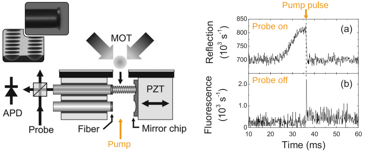
Figure 1.5: The microcavity QED experiment at CCM. Left, the experimental set-up. Micrographs of the fibered mirror and of the spherical micromirrors array are shown in inset. Right: Experimental results. Ground state Rb atoms are dropped from a MOT and fall freely through the cavity mode; the passage of a single atom disturbs the cavity, as seen in the change in the reflection of a probe beam in the first half of trace (a). The maximum mean atom number is \langle n \rangle \simeq 1 . At the time indicated by the vertical dashed line, the atoms are excited by the pump laser shown in the diagram (left) into the excited state; a sharp burst of cavity-enhanced photon is then observed through the fibre (b). About 50% of the photons are emitted into the cavity mode, indicating a cooperativity C \sim 1 . Graphics adapted from (71).
