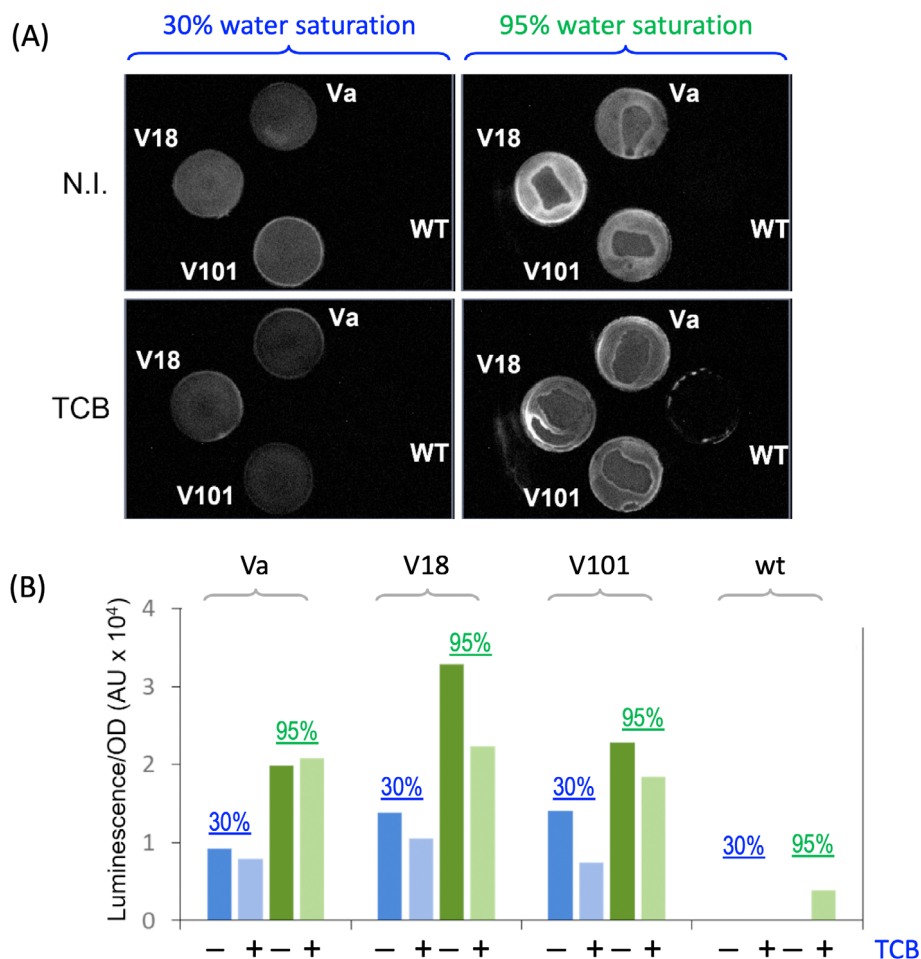
FIGURE 4 Activation of four biosensor strains with XylR A domain variants or wild type tested on 0.22 µm filters exposed to two different humidity levels. The figure shows the transcriptional activation of the Pu promoter in four P. putida biosensor strains with wild-type XylR A domain or with A domain variants Va (M14I, I129N), V18 (S47R, L110S), or V101 (Y159F, L222R) on filters in low (30%, blue bars) or high (95%, green bars) humidity when induced or not with TCB as indicated. Variants of the XylR A domain gene were inserted in the attTn7 site of a P. putida host with a Pu-lux cassette.
