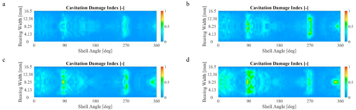
Fig. 7. Cavitation Damage Index contour plot obtained with the presented procedure for the steel connecting rod at 8500 rpm (a), 10500 rpm (b), 11500 rpm (c) and 12500 rpm (d).
