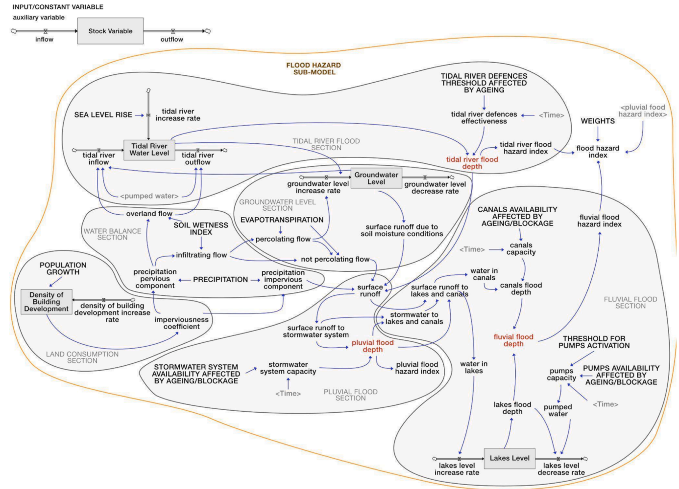
Fig. 3. Thamesmead 'Flood hazard' sub-model. Sub-model parts are represented with grey circles. Variables in capital letters are the main inputs of the simulation, while variables in red are the main outputs in terms of simulated flooding mechanisms. (For interpretation of the references to colour in this figure legend, the reader is referred to the web version of this article.)
