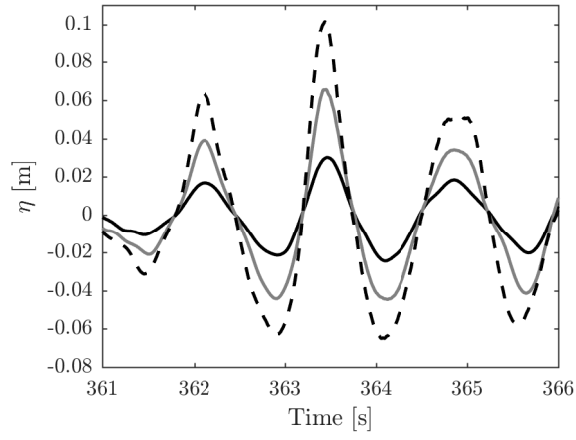
FIG. 2. Segment of time-histories that demonstrate the wave generation method and relate to the same seed in sea-states with: S_p = 0.01 [black line], S_p = 0.02 [grey line] and S_p = 0.03 [dashed line]; all with \sigma_\theta = 10^\circ .
