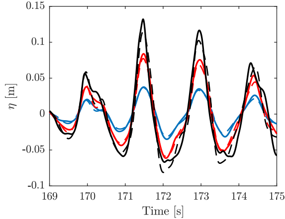
(a) k_p d : 1.02 and \sigma_\theta : 10^\circ
