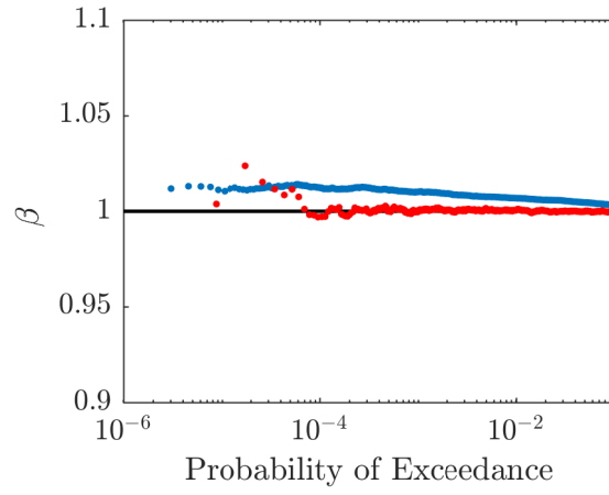
FIG. 14. Distribution of the front-back wave trough ratio ( \beta ) corresponding to all sorted wave heights arising in field measurements water depths of d = 45 m [red] and d = 7.7 m [blue].
