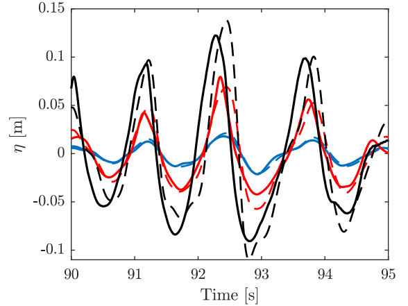
(b) k_1 d : 1.22 and \sigma_\theta : 10^\circ
