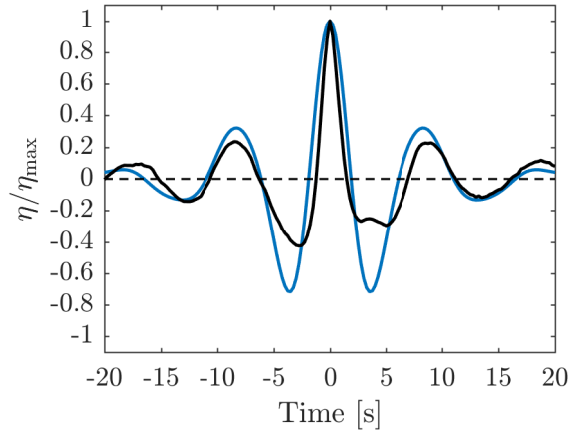
(e) Field data: H_s = 2 m, T_p = 8 s, d = 7.7 m
