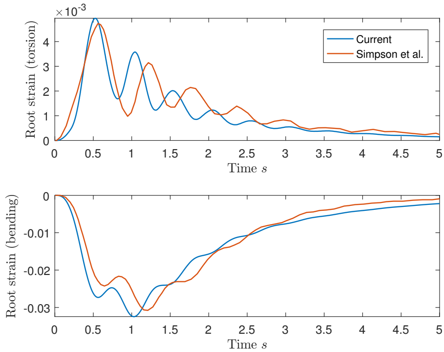
Figure 7.3: Root strains of the Long-Goland wing due to gust input described in (7.3), with L_{GU} = 20\text{ m} and w_0 = 17.07\text{ m s}^{-1} . The blue line is the current implementation and the red line is taken from Figure 12 by Simpson et al. [62].
