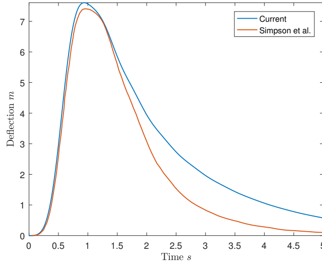
Figure 7.2: Tip displacement of the Long-Goland wing due to gust input described in (7.3), with L_{GU} = 20\text{ m} and w_0 = 17.07\text{ m s}^{-1} . The blue line is the current implementation and the red line is taken from Figure 11 by Simpson et al. [62].
