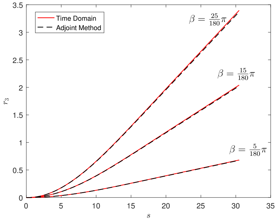
Figure 7.4: Steady state displacement in the \mathbf{e}_3 direction over the span of Long-Goland wing due to the control surface defined in (7.1.4) with deflection \beta .
