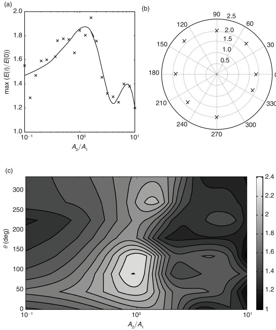
Figure 17: Variation of the maximum energy amplification E_{\max} with (a) amplitude ratio A_2/A_1 for fixed phase angle \theta = 0^\circ and (b) with phase angle \theta for fixed amplitude ratio A_2/A_1 = 1 . The symbols (x) indicate the experimental data point; the continuous line represents a Gaussian fit. (c) Maximum transient growth over initial conditions of the form A_1 \sin(2\pi f_1 t) + A_2 \sin(2\pi f_2 t + \theta) . The optimal initial condition for maximum transient growth is identified for the parameter combination A_2/A_1 = 0.93 and \theta = 90^\circ . The corresponding maximum transient growth is 2.3. The remaining parameters are f_1 = 173 \text{ Hz} , f_2 = 346 \text{ Hz} , \dot{m} = 2.34 \text{ g/s} and k = 747 \text{ W} .
