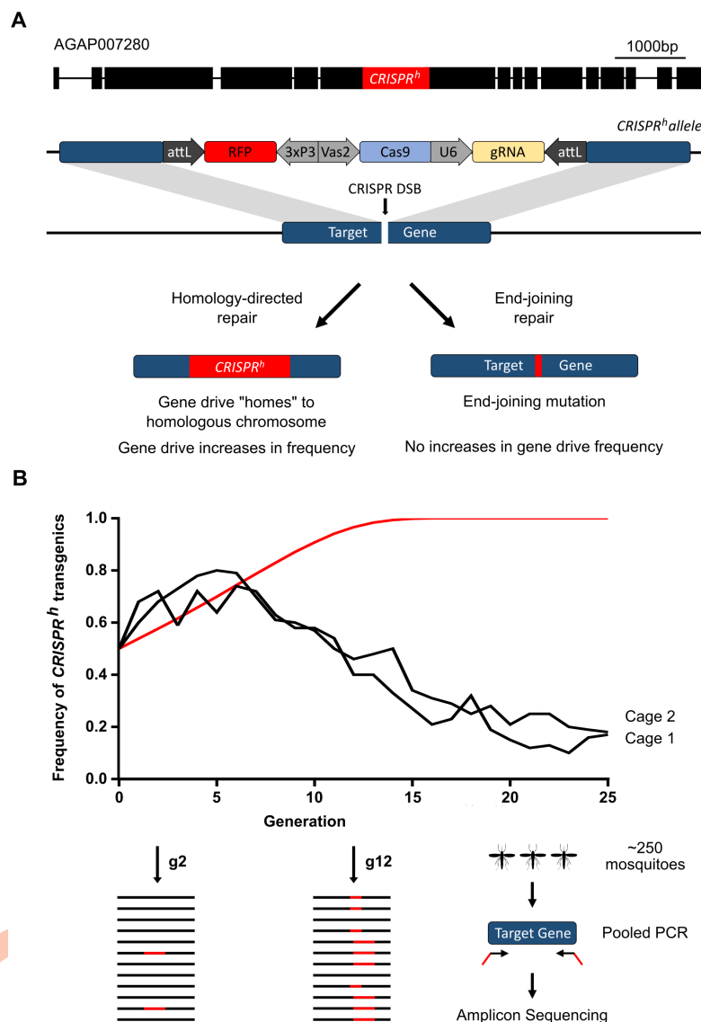
Fig 1. Dynamics of a population suppression gene drive construct over 25 generations. (A) Design of the CRISPR-based gene drive construct and the relevant position of its target site within AGAP007280; (B) The proportion of individuals containing at least one copy of the gene drive in two replicate cages, monitored each generation for 25 generations. Black lines represent the observed frequencies in each of the two cage trials (CT1 and CT2), red line represents the predicted frequency according to the previous deterministic model that did not take into account target site resistance [11]. Samples were taken for pooled PCR and sequencing analysis of the gene drive target site at G 2 and at G 12 , whereby frequency of target site indels (shown figuratively as red bars) were revealed by their relative representation among the sequenced reads.
