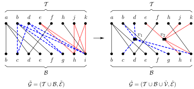
Fig. 3 Compression of \tilde{\mathcal{G}} into \hat{\mathcal{G}} via edge concentration
