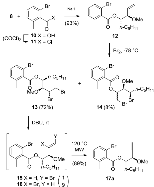
Scheme 2. Formation of alkyne 17a .
