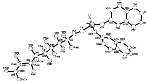
Figure 3. Molecular structure of germyl hydride 27 [HGe(CH 2 -2-Nap) 2 (CH 2 ) 2 C 8 F 17 ] (X-ray)
