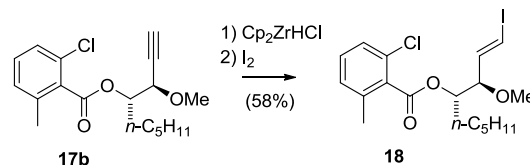
Scheme 4. Formation of alkenyl iodide 18 .
