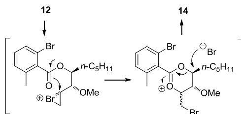
Scheme 3. Plausible pathway for formation of 1,4-dibromide 14 .
